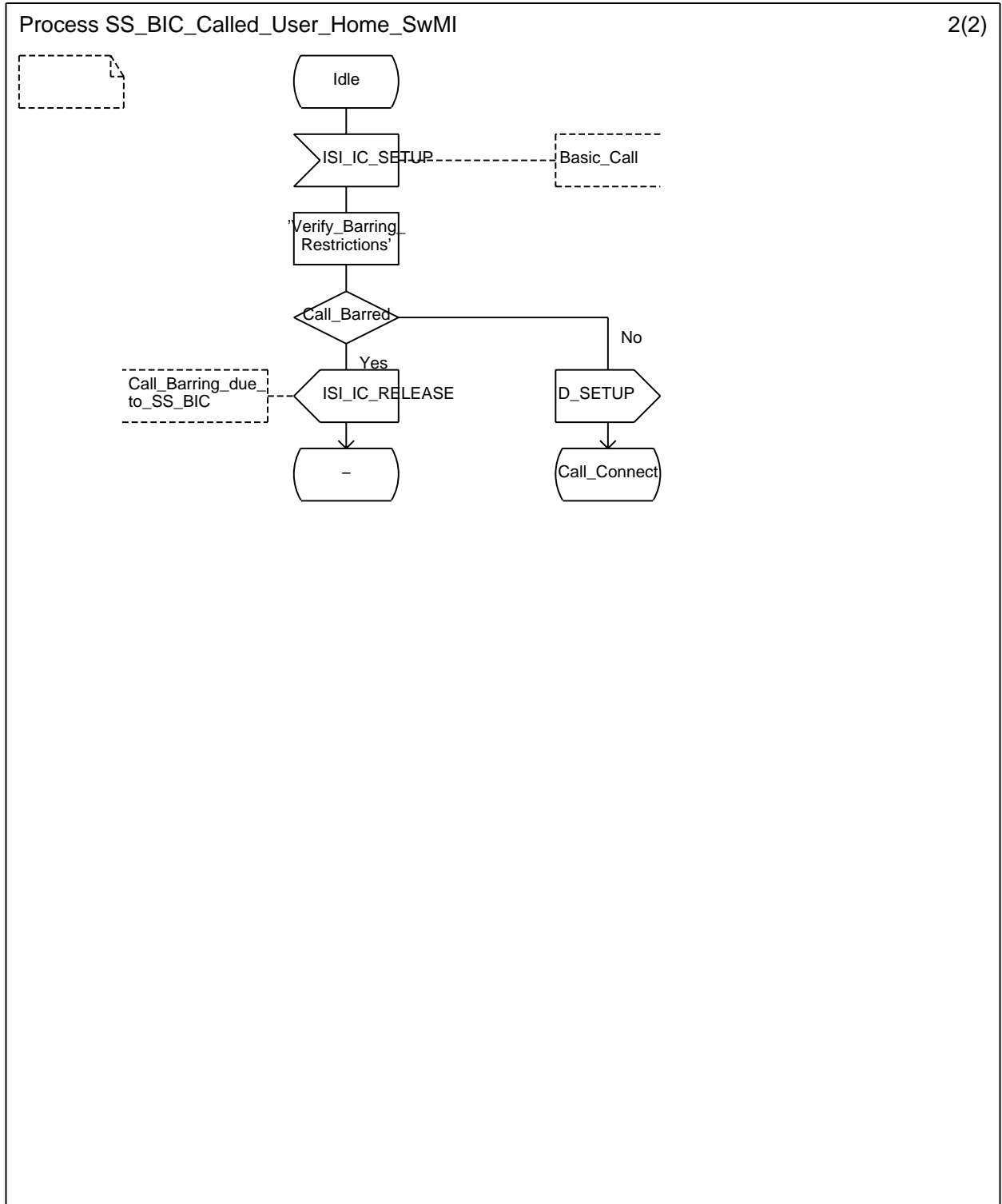
Figure A.5: SDL representations of SS-BIC at SS-BIC called user home SwMI (2/2)
