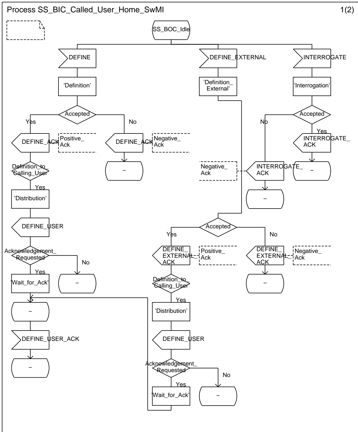
Figure A.5: SDL representations of SS-BIC at SS-BIC called user home SwMI (1/2)
