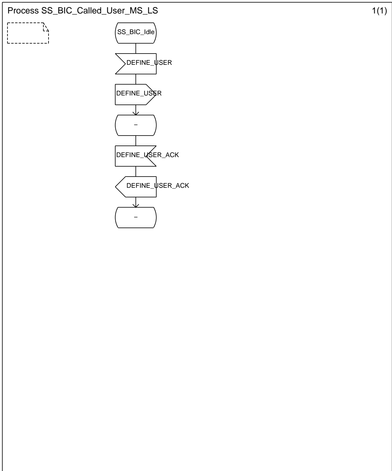
Figure A.6: SDL representations of SS-BIC at SS-BIC called user MS/LS
