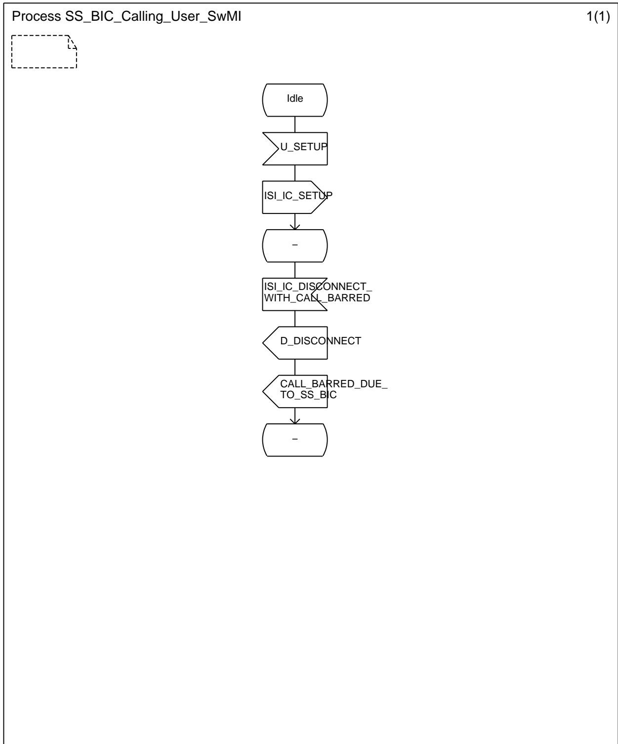
Figure A.2: SDL representations of SS-BIC at calling user home SwMI
