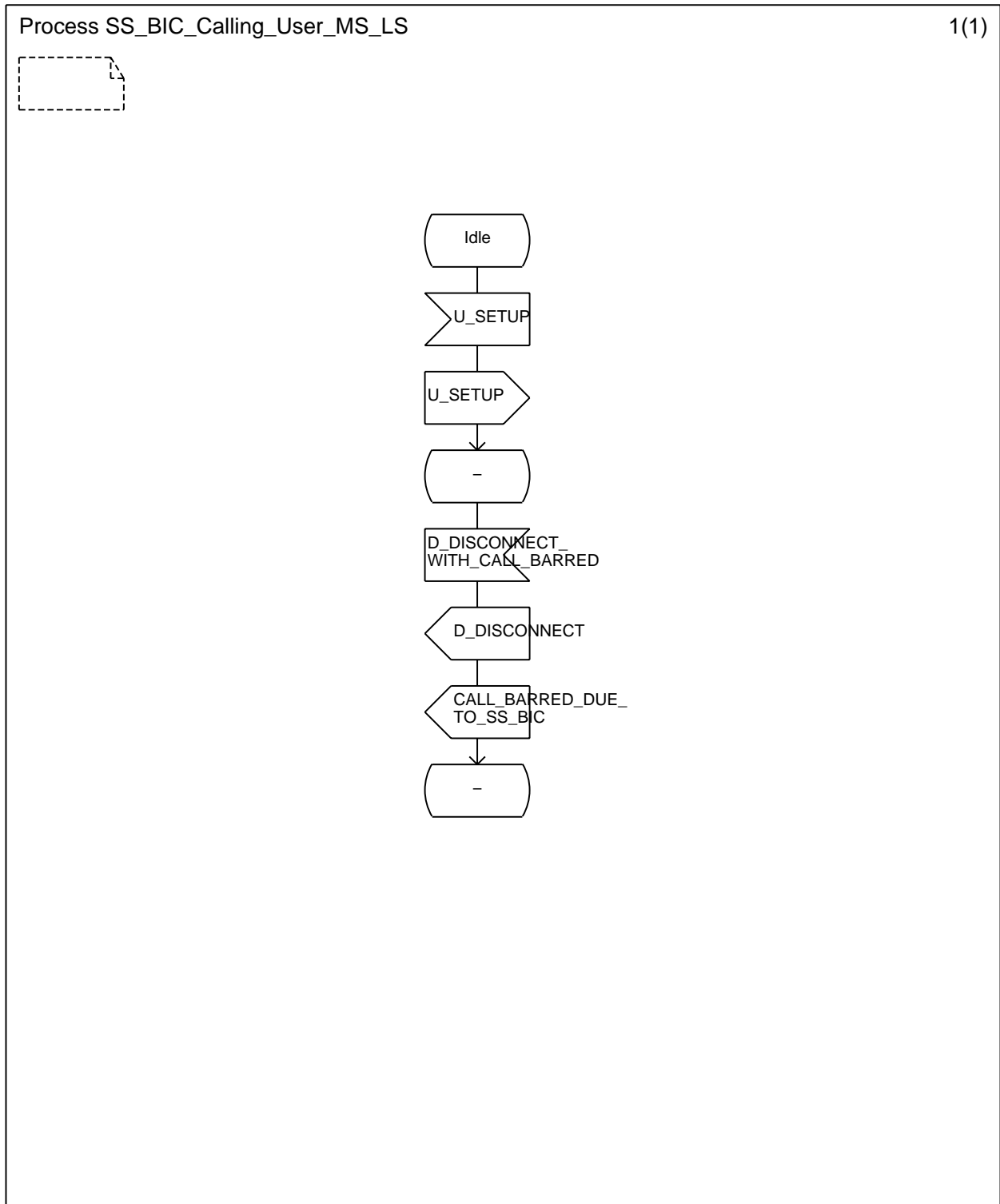
Figure A.1: SDL representations of SS-BIC at calling user MS/LS
