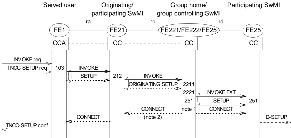
Figure 14: Basic invocation and operation of SS-AS over ISI - successful establishment of group call when the selected area definition is given in the group home SwMI and no SS-AS inhibition for calling user with the originating SwMI lying partly within the selected area
