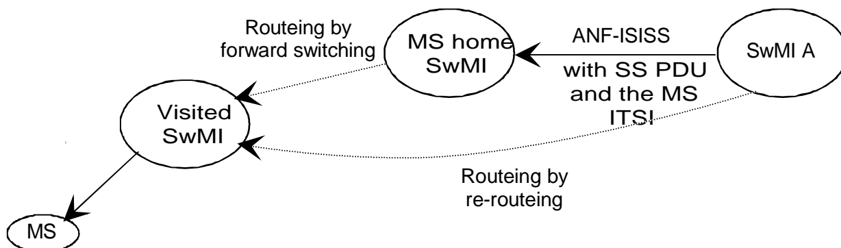
Figure 3: SS PDU addressed individually by an SwMI to an MS/LS
