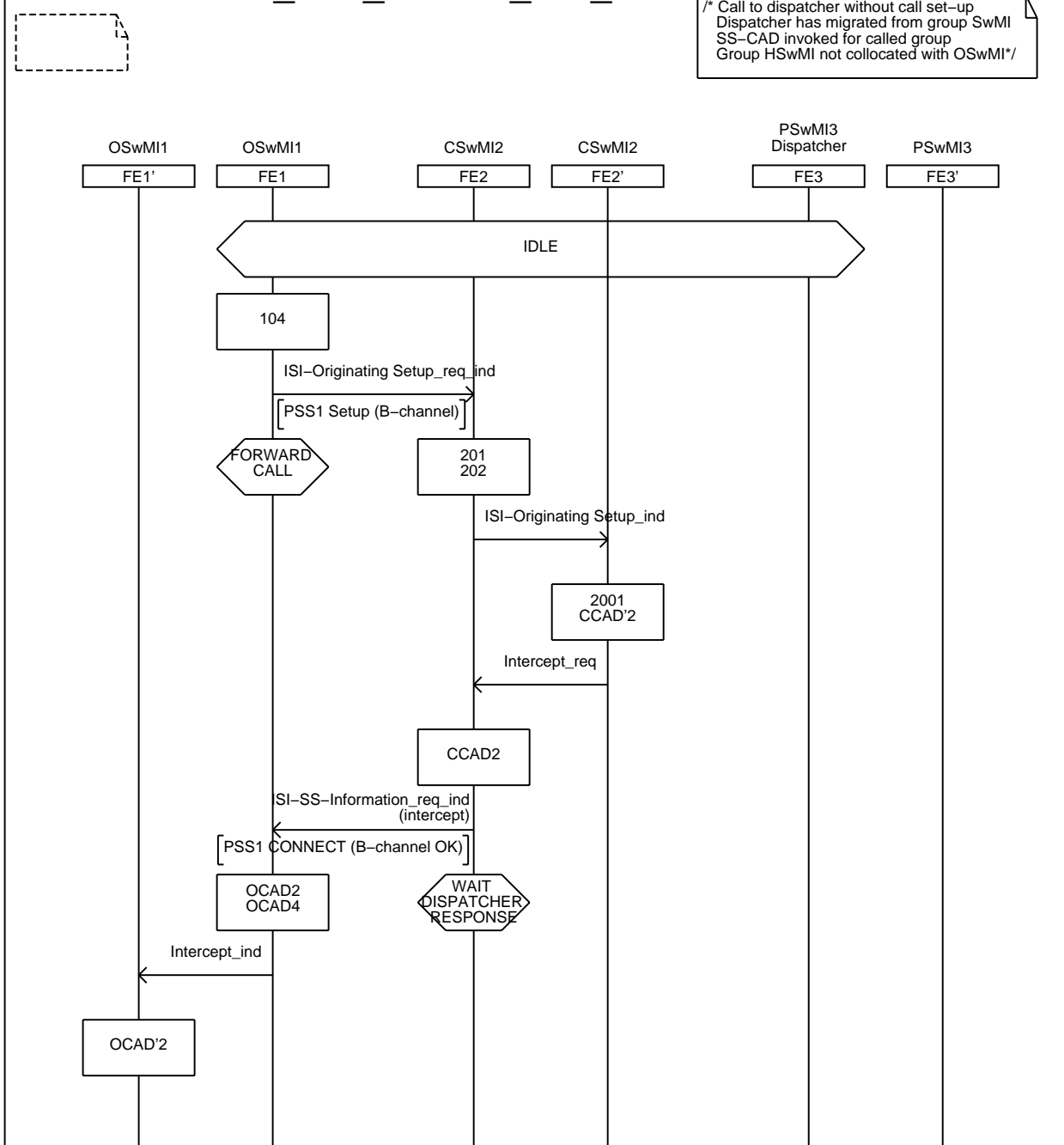
Figure B.6: Information flow sequence - Call to dispatcher without call set-up (sheet 1 of 3)
