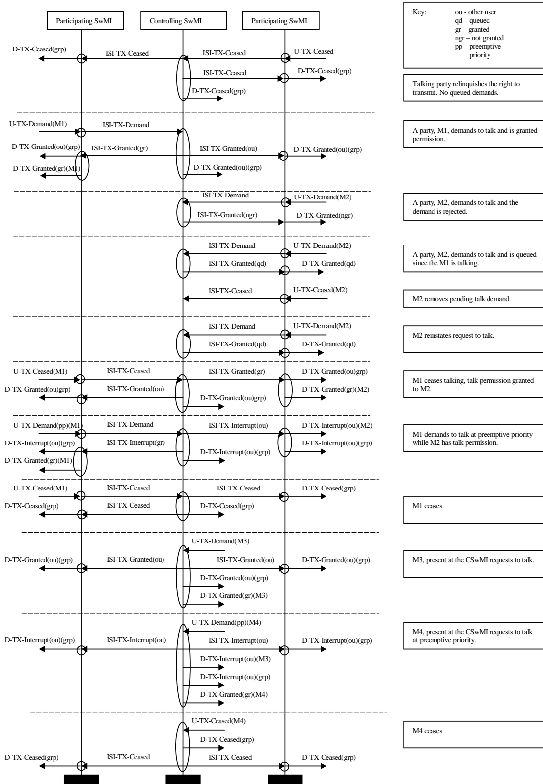
Figure E.24: Call maintenance
