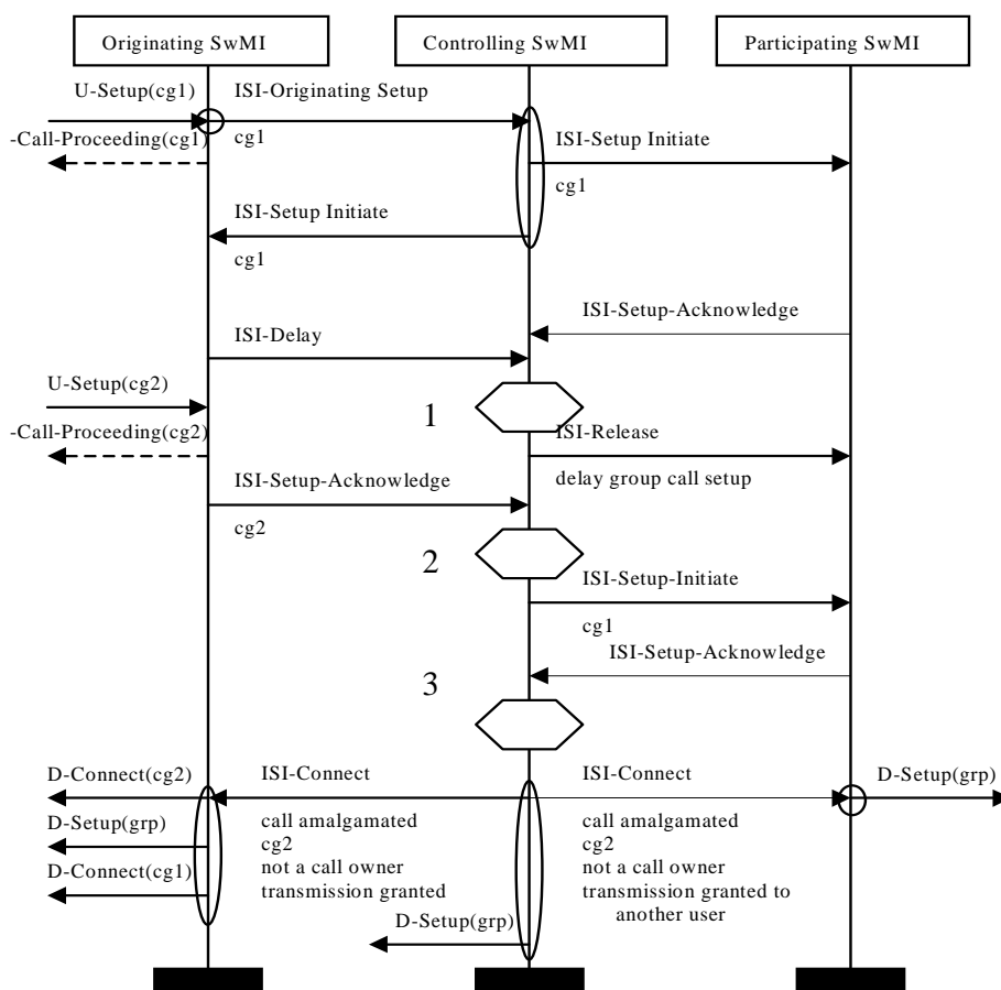
Figure E.13: Successful group call set-up: multiple calling parties at the same SwMI
