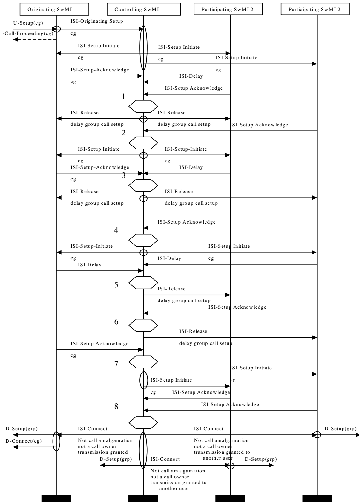
Figure E.4: Successful group call set-up: single calling party, some queuing for resources, showing multiple releasing
