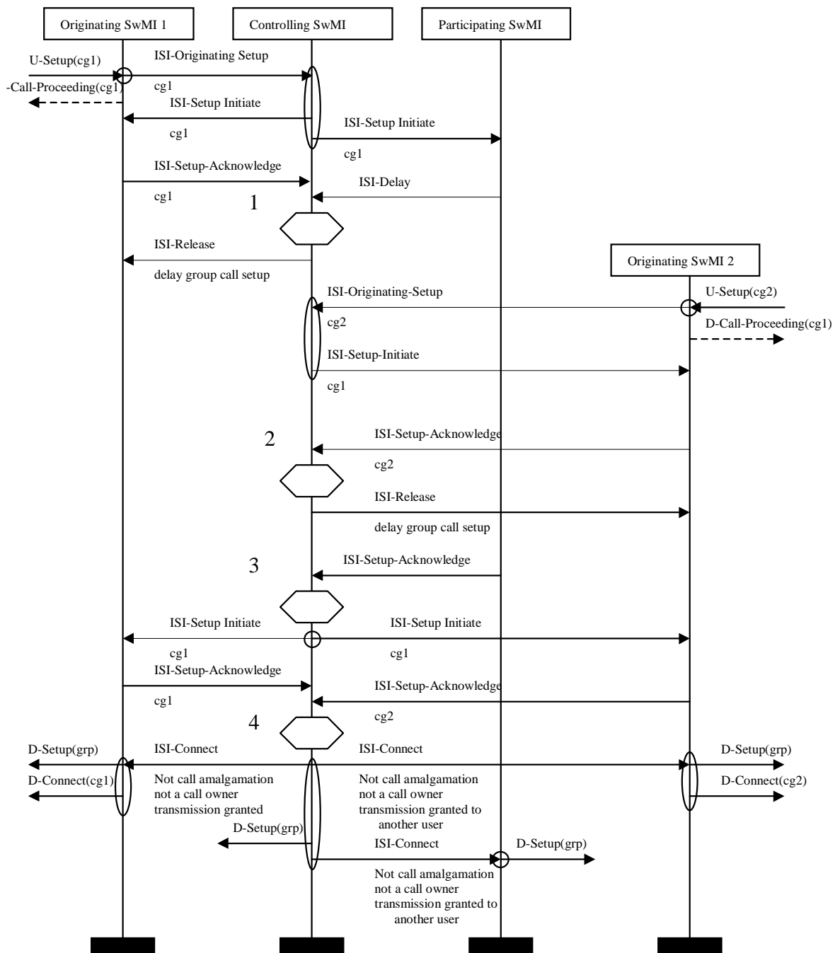
Figure E.8: Successful group call set-up: multiple calling parties the second calling OSwMI is ready first
