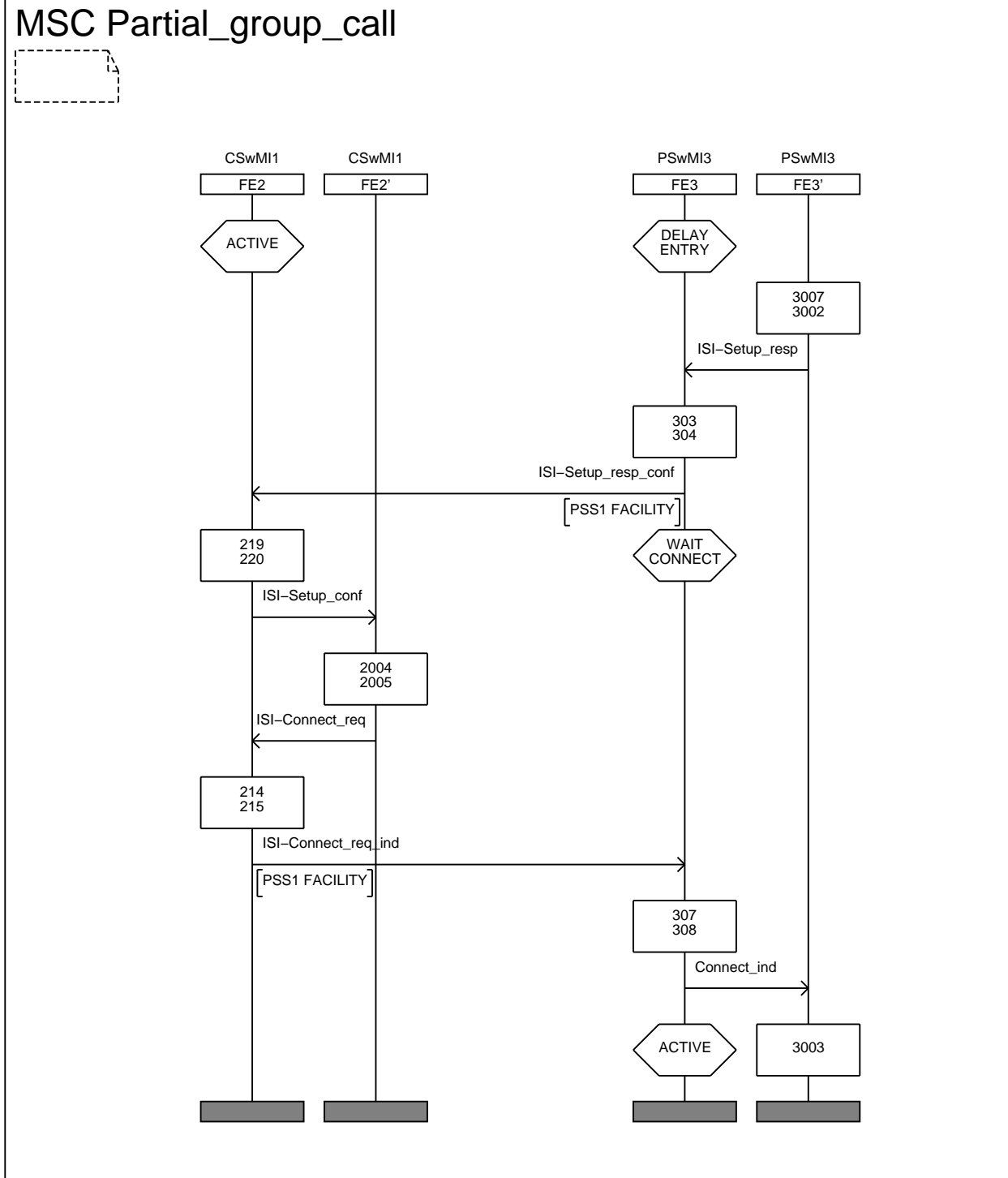
Figure 34: Information flow sequence - partial group call set-up (sheet 3 of 3)
