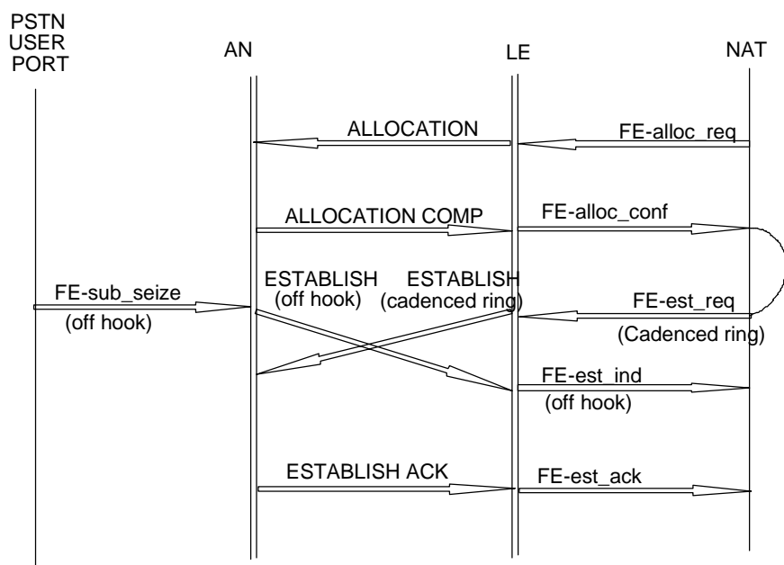
Figure E.14: PSTN call collision, terminating call has priority
