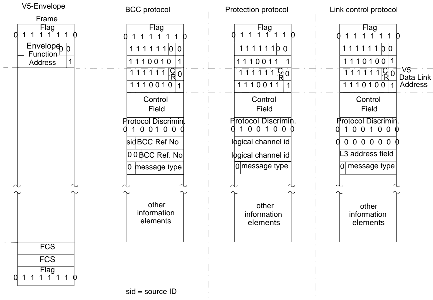
Figure M.2: Additional frame formats used in the V5.2 interface
