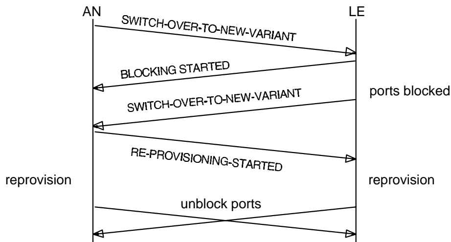
Figure C.2: Procedure for re-provisioning initiated from AN
