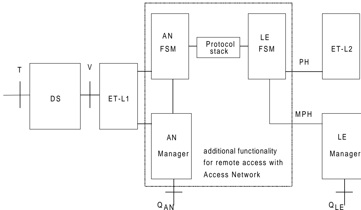
Figure 3: ISDN user port functional model
