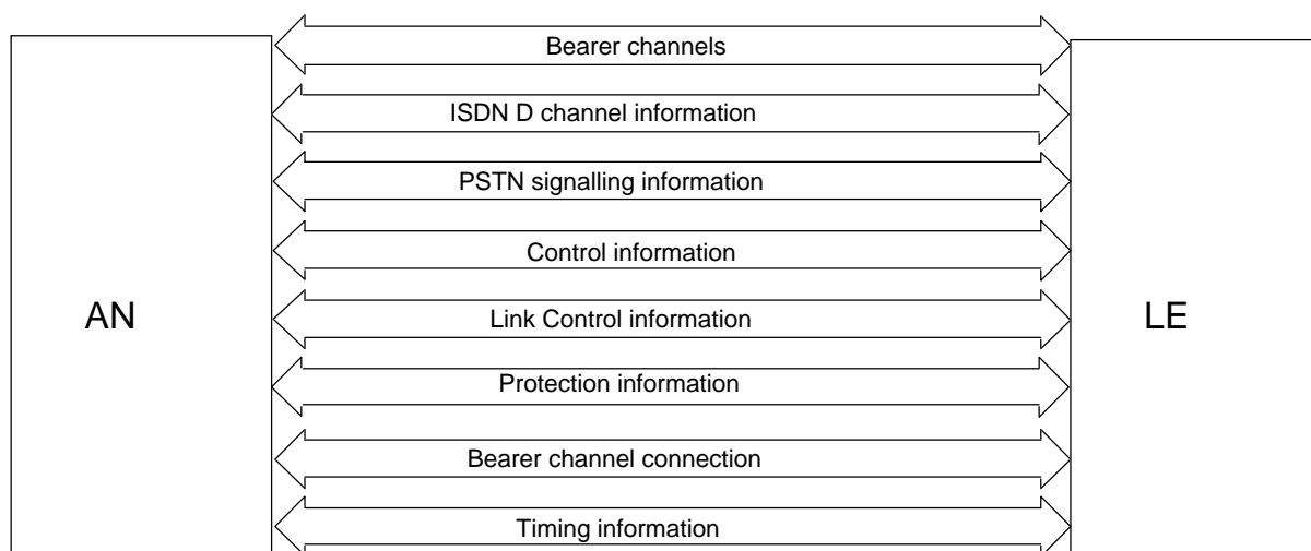
Figure 5: Functional description of the V5.2 interface
