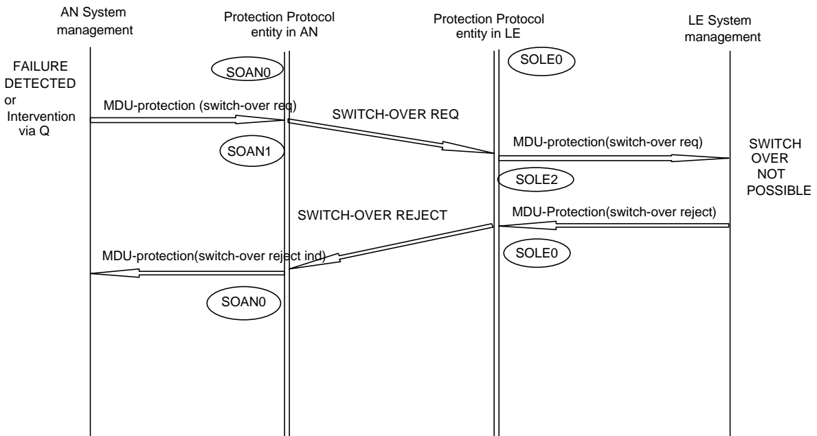
Figure P.4: Rejection of AN-initiated switch-over by LE
