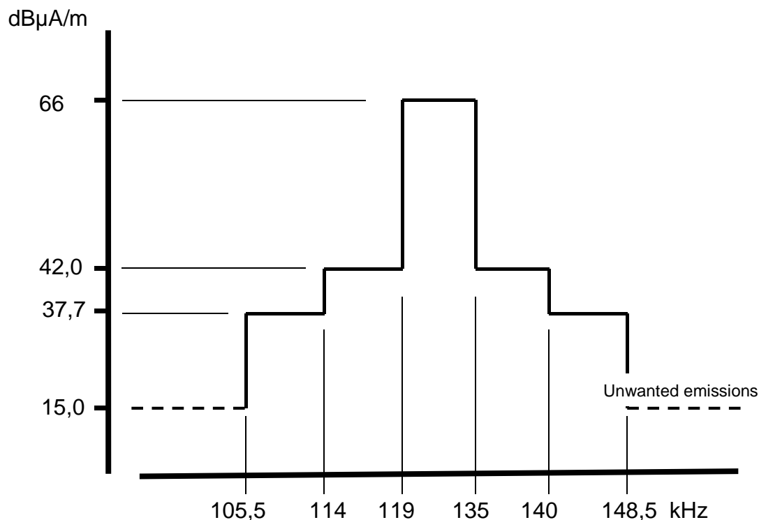
Figure G.1: Emission boundary for LF RFID systems
