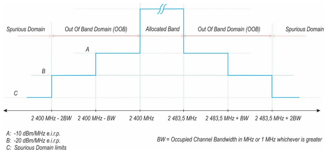
Figure 1: Transmit mask
