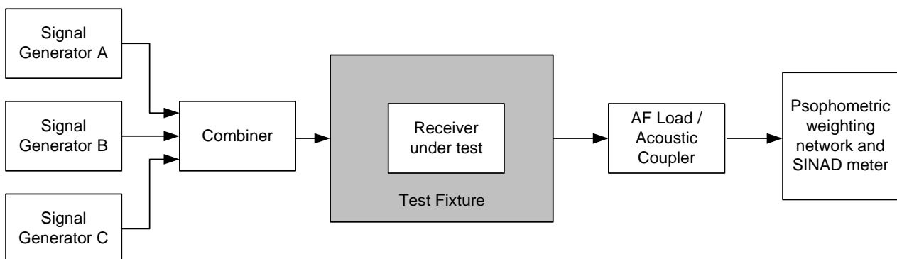
Figure 18: Measurement arrangement
