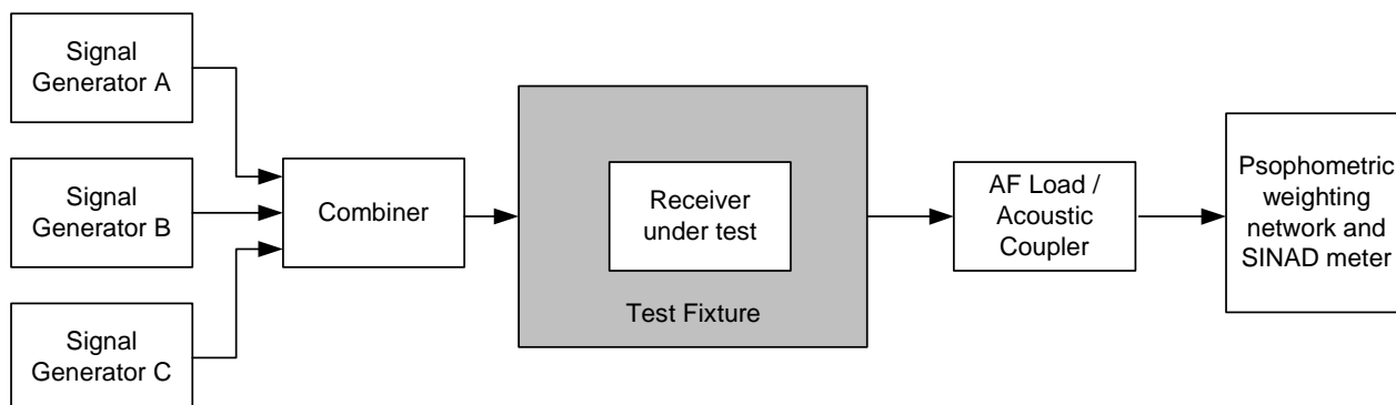
Figure 18: Measurement arrangement
