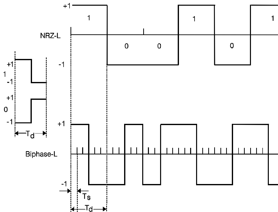
Figure 2: Example of bi-phase-L coding
