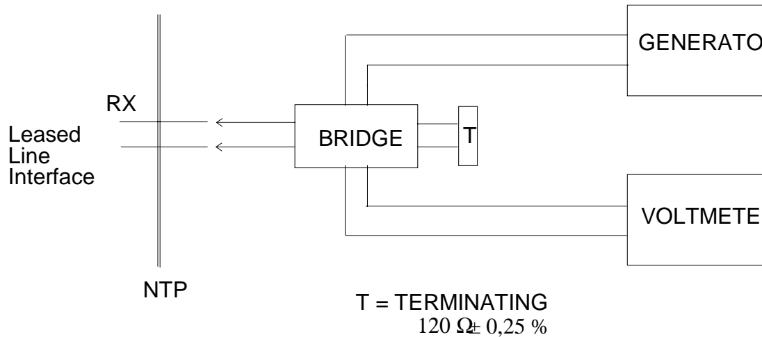
Figure A.5: Return loss at input port
