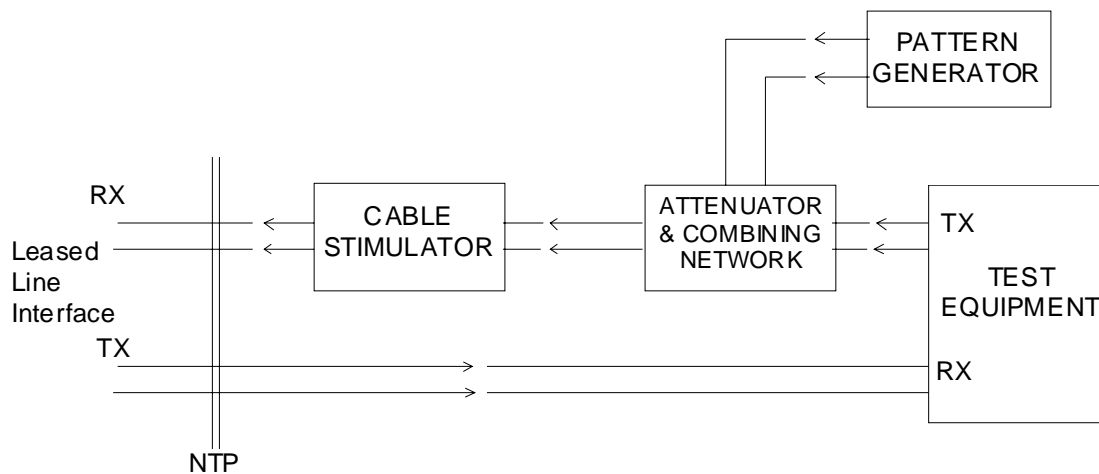
Figure A.4: Immunity against reflections
