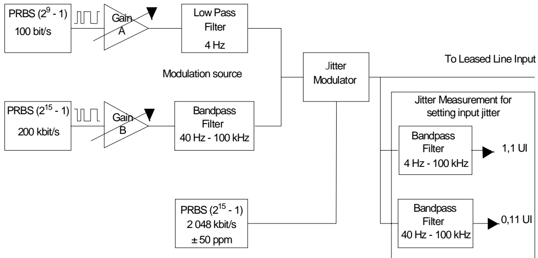
Figure A.4: Input jitter generation
