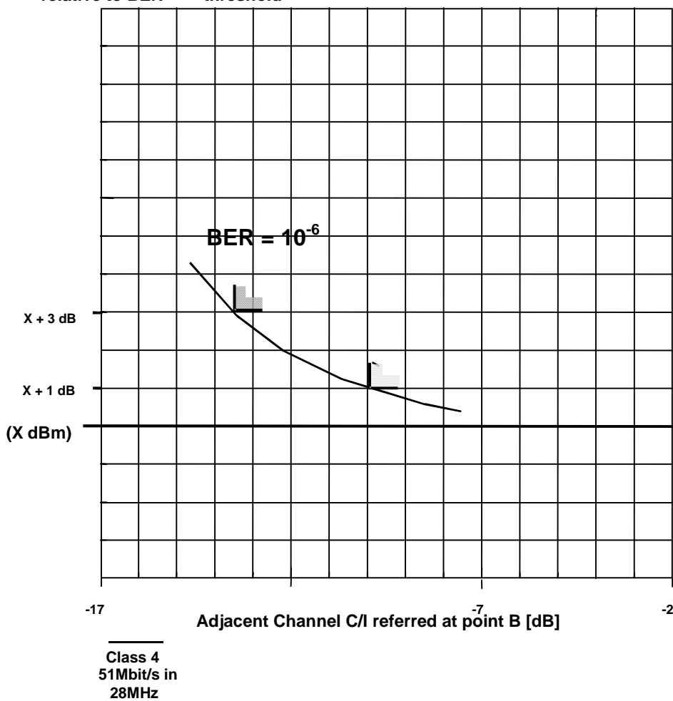
Figure A.5: First adjacent channel interference threshold degradation
