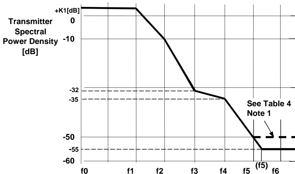
Figure 3b: Limits of spectral power density for class 3 systems
