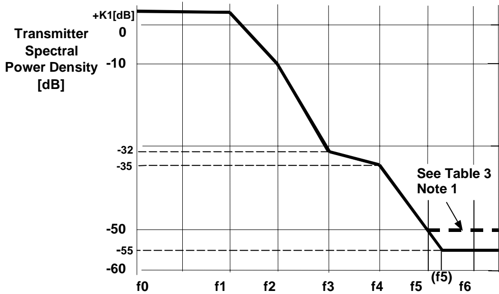
Figure 3c: Limits of spectral power density for Class 5a systems
