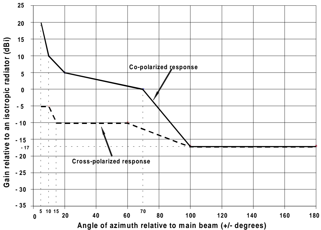
Figure A.2 c): Type C antenna radiation pattern (under test conditions)
