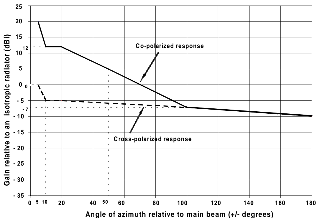
Figure A.2 a): Type A antenna radiation pattern (under test conditions)
