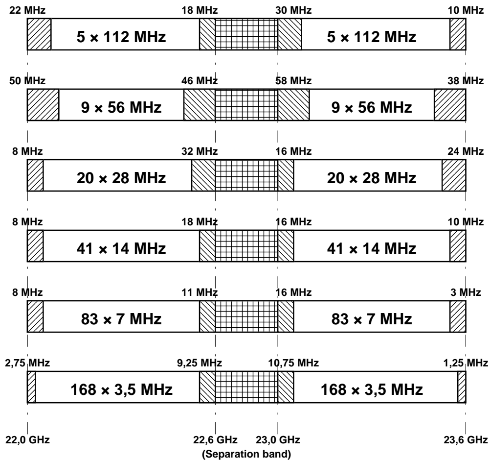
Figure A.1: Radio frequency channel arrangement
