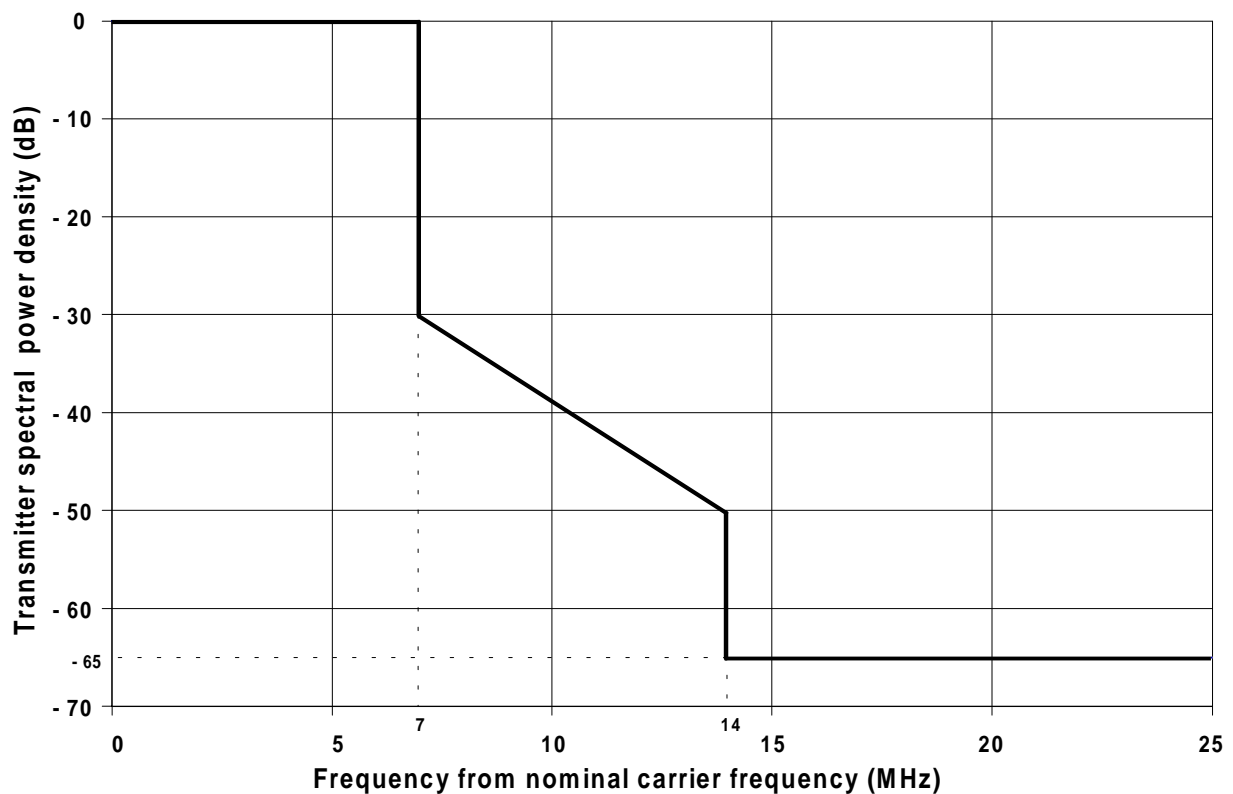
Figure 3: Limits of spectral power density for video basebands up to 3,5 MHz (using channel spacing of 28 MHz - referred to nominal centre frequency (fo))
