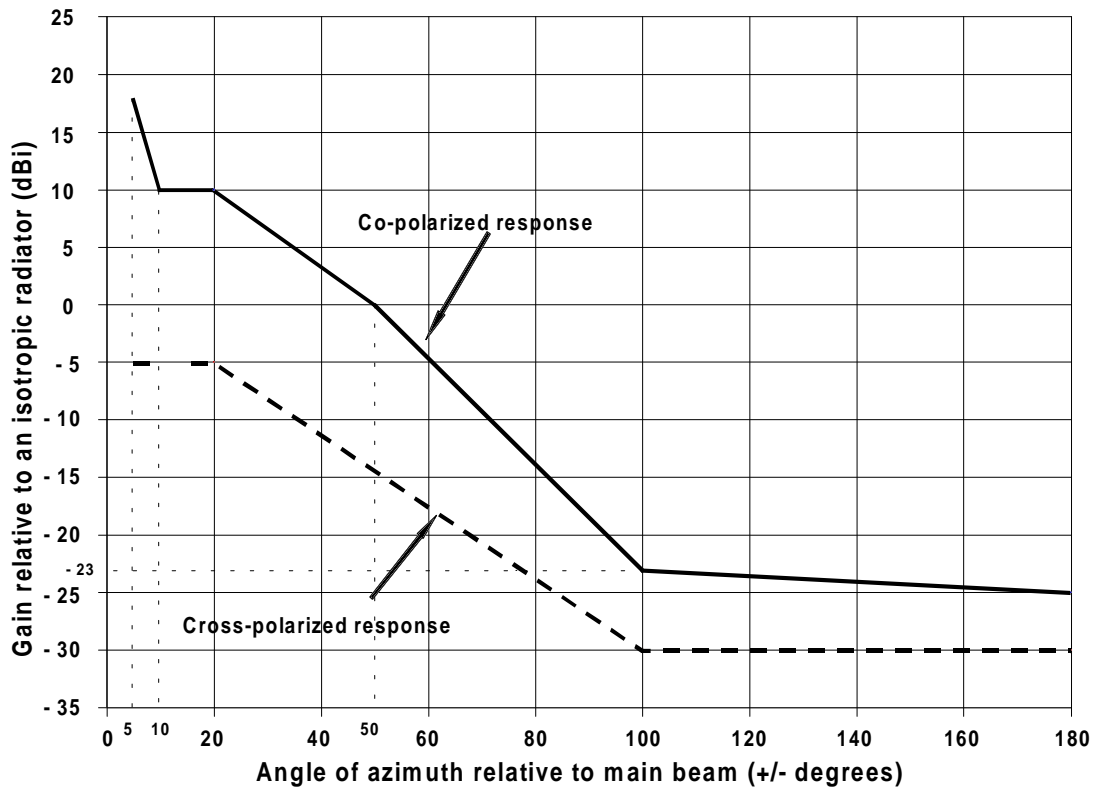
Figure A.2 b): Type B antenna radiation pattern (under test conditions)
