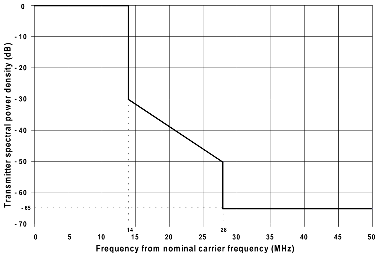
Figure 4: Limits of spectral power density for video basebands up to 14 MHz (using channel spacing of 56 MHz - referred to nominal centre frequency ( f_0 ))
