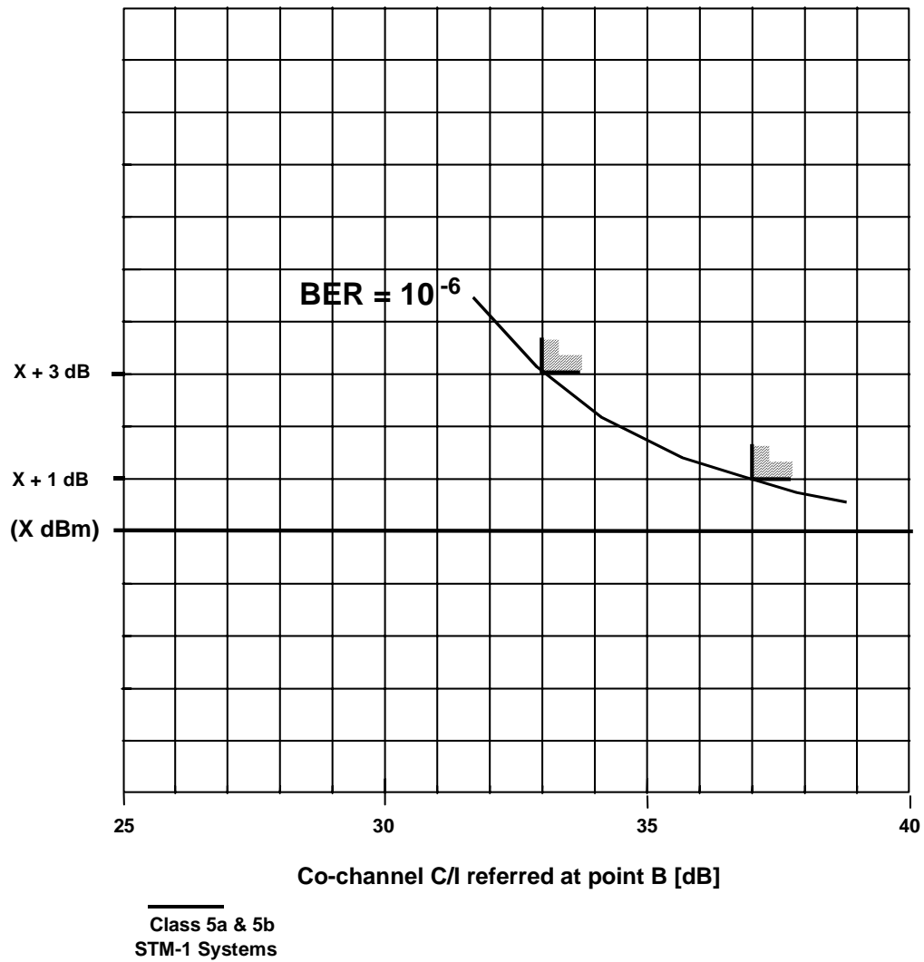
Figure A.5.1b: Co-channel interference threshold degradation
