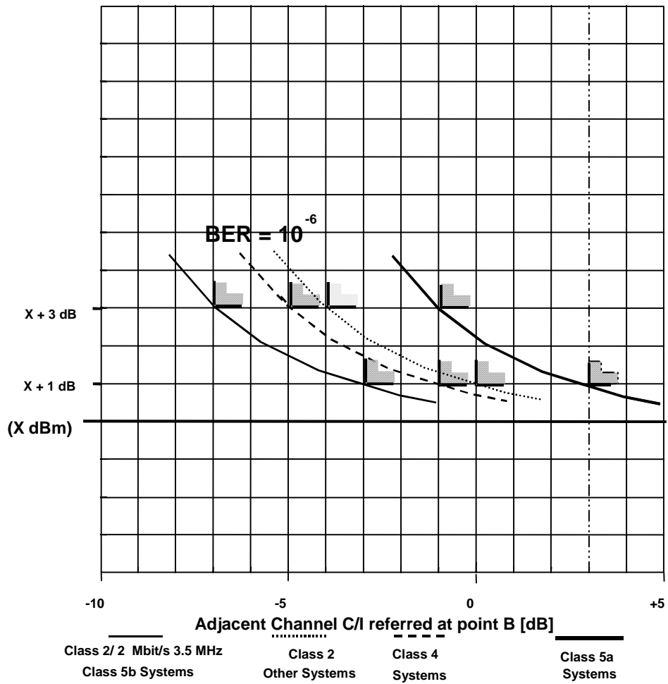
Receiver Input Level at Reference Point C relative to BER -6 threshold
