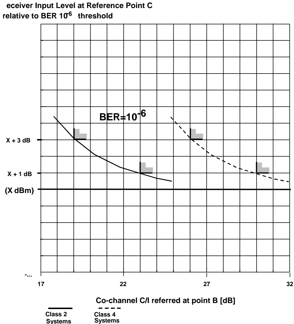
Figure A.5.1a: Co- channel interference threshold degradation
