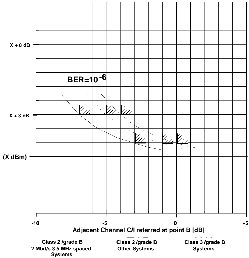
Figure A.3.2: First adjacent channel interference threshold degradation
