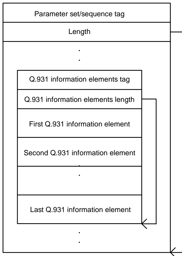
Figure H.1: Encapsulation of Q.931 information elements
