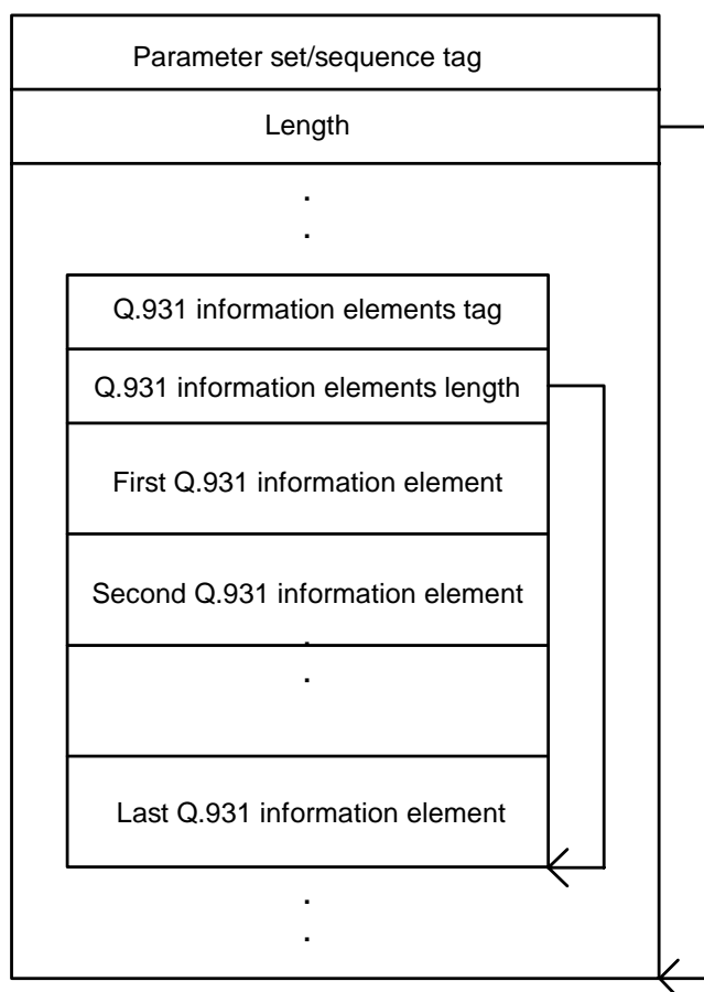
Figure H.1: Encapsulation of Q.931 information elements
