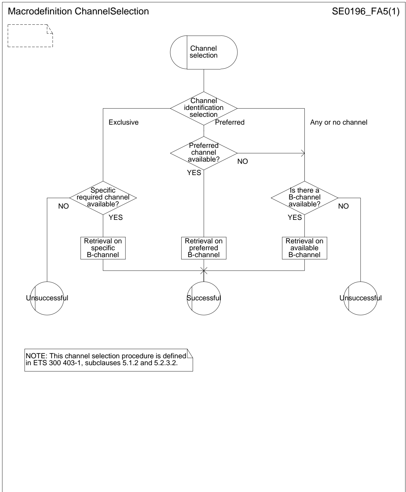
Figure A.5: SDL diagram of channel selection macro
