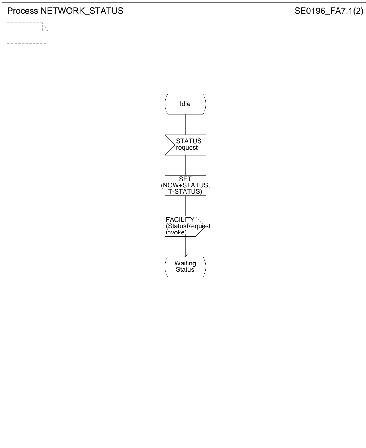
Figure A.7 (sheet 1 of 2): Status request procedure - network SDL diagrams
