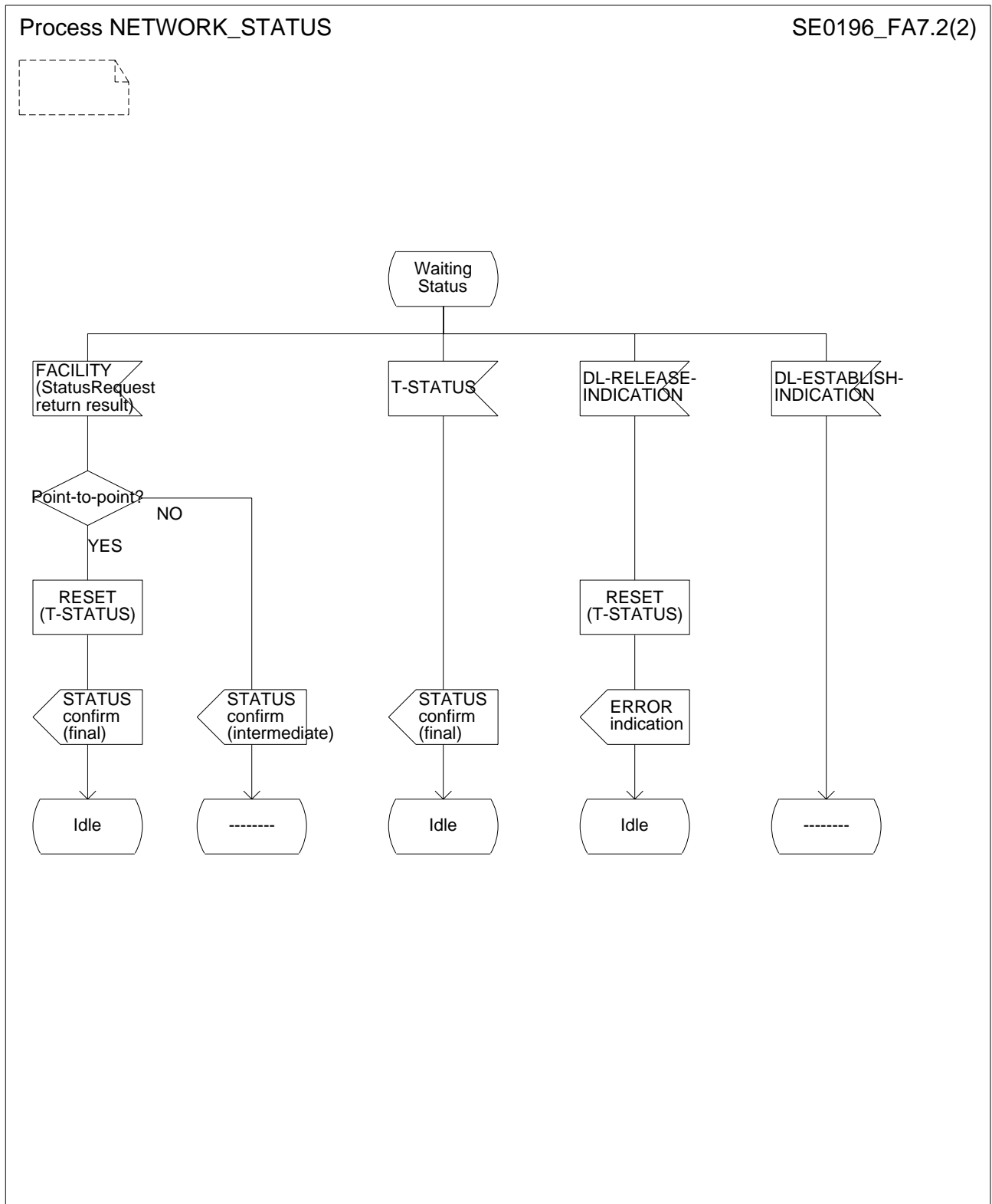
Figure A.7 (sheet 2 of 2): Status request procedure - network SDL diagrams
