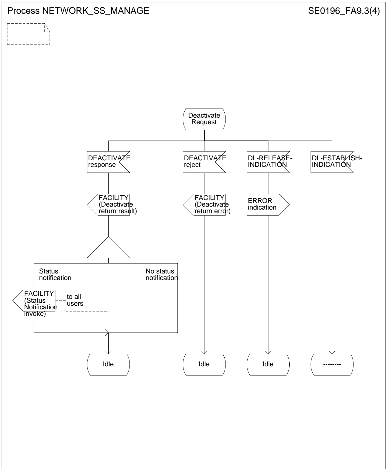
Figure A.9 (sheet 3 of 4): Supplementary service management procedures - network SDL diagrams
