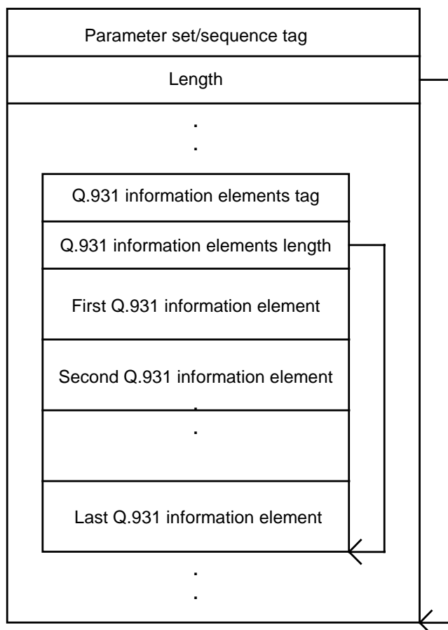
Figure H.1: Encapsulation of Q.931 [20] information elements
