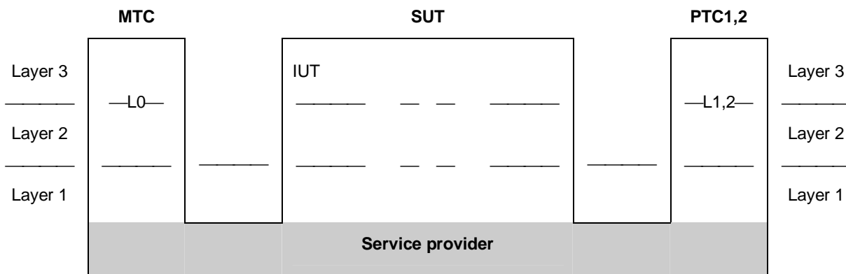
Figure 2: Combination of the remote and multi-party test methods
