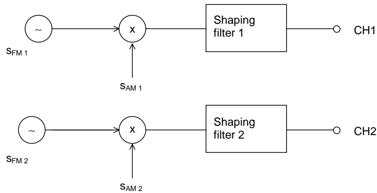
Figure 7.10c: Measurement signals
