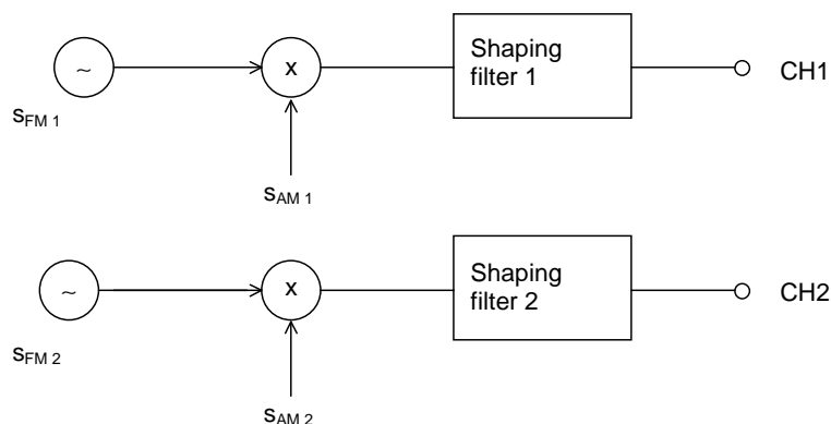
Figure 7.14d: Measurement signals
