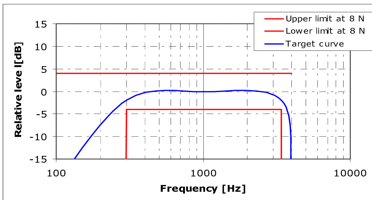
Figure 7.4: Receive frequency response mask for 8N application force
