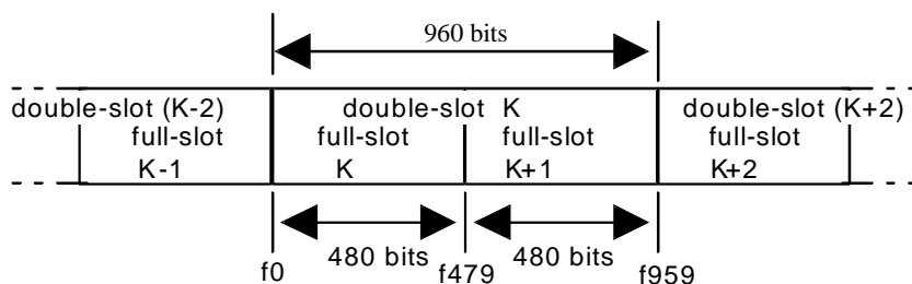
Figure 26: Double-slot format
