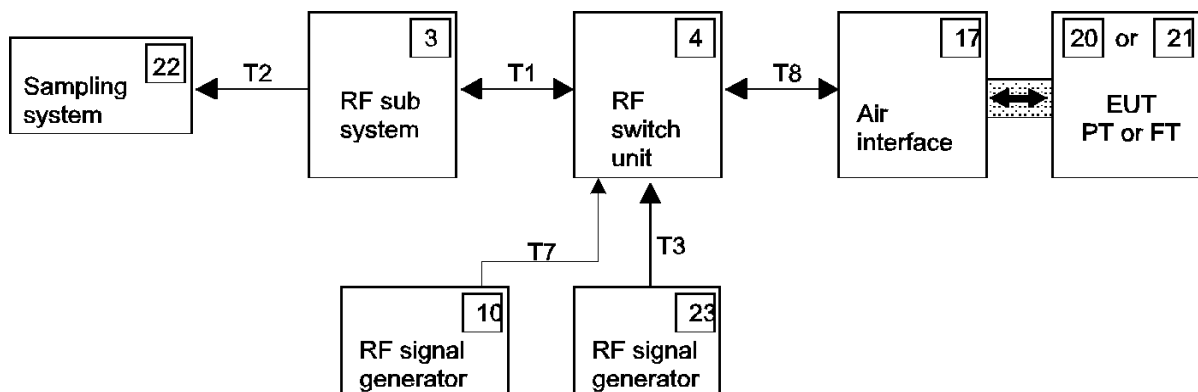
Figure 12: Test setup 3
