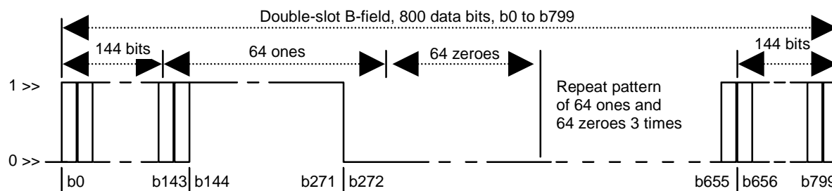
Figure 32: Test packet transmission for case 2, full-slot
