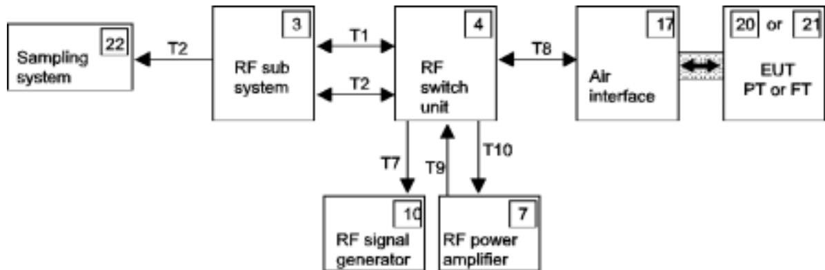
Figure 14: Test setup 5
