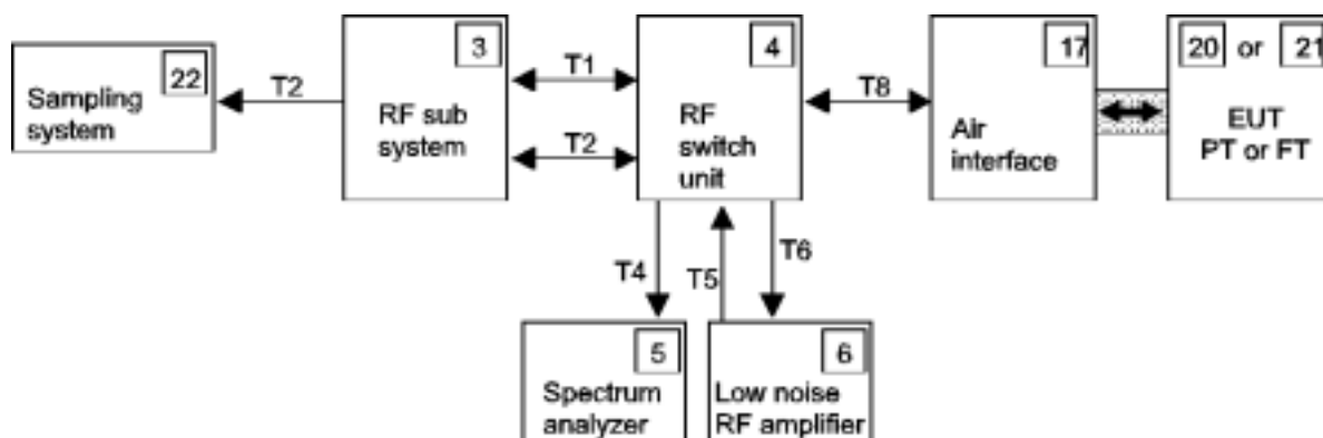
Figure 13: Test setup 4
