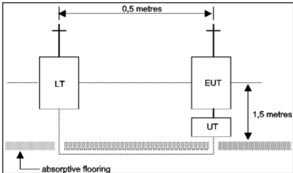
Figure 15: Test arrangement
