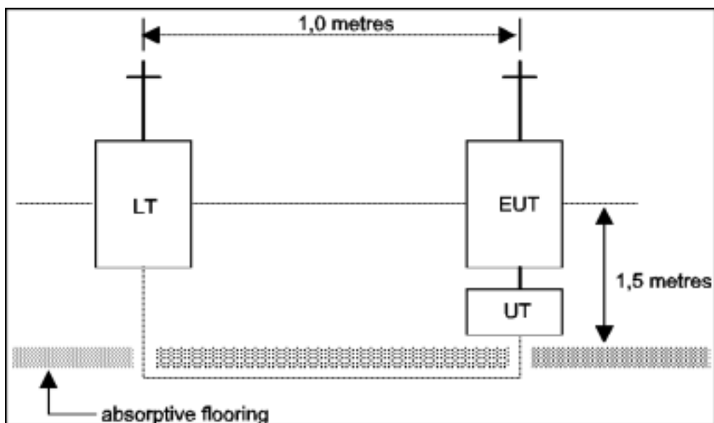
Figure 17: Test arrangement
