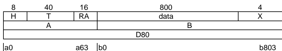
Figure 6.12: Double slot field structures
