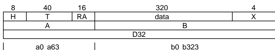
Figure 6.2: Field structures
