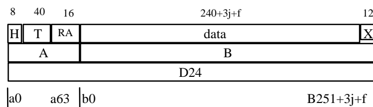
Figure 6.15 (continued): Unprotected B-field slot field structures for 4- and 8- level modulation slot formats
