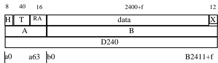
Figure 6.15 (concluded): Unprotected B-field slot field structures for 4- and 8- level modulation slot formats
