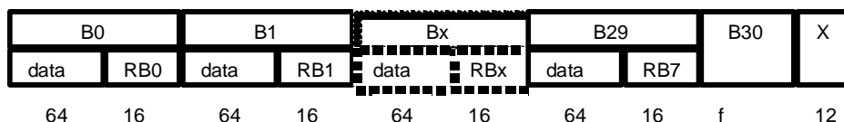
Figure 6.16: B-field multisubfield protected format for 4- and 8 level modulation formats
