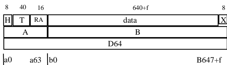
Double slot, 4 level modulation
