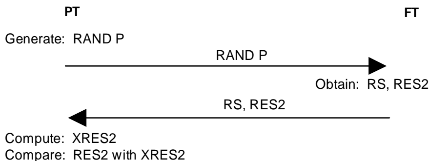
Figure 4.2: Authentication of FT
