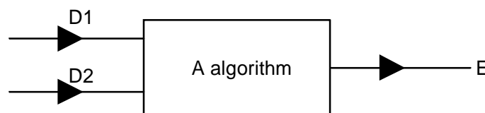
Figure 5.1: A algorithm
