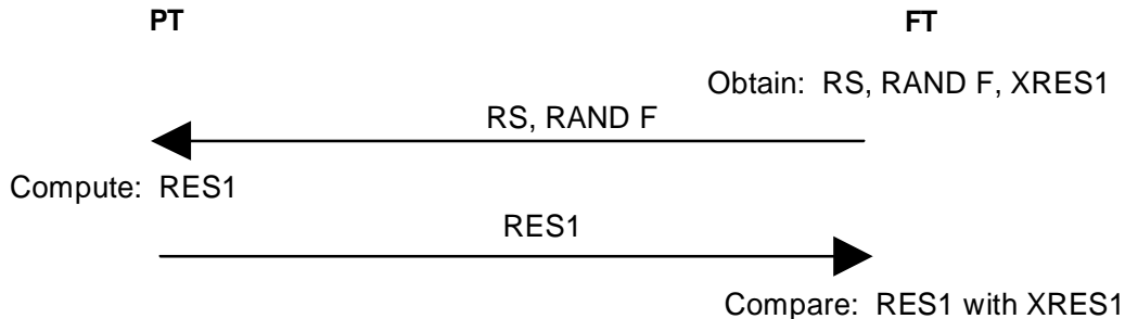
Figure 4.1: Authentication of PT
