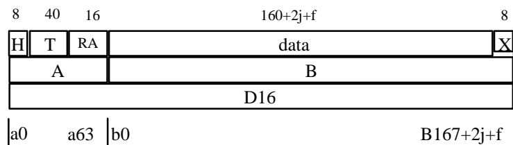
Full slot, 4 level modulation
