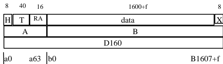
Half slot, 8 level modulation
