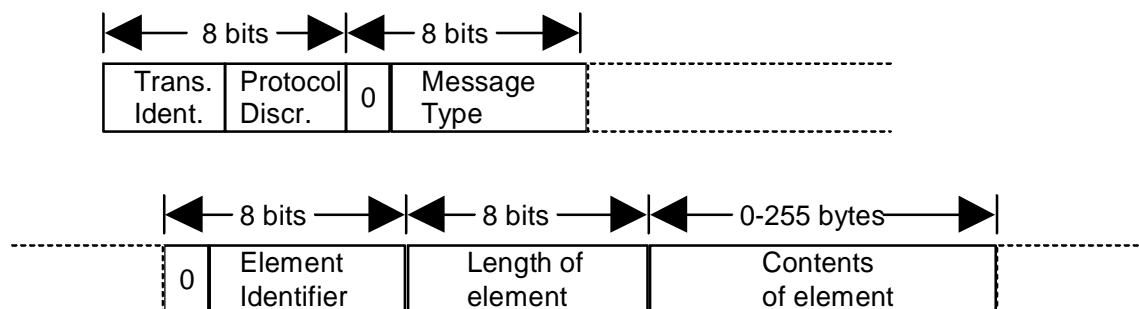
Figure 6.1: NWK Layer Message Structure (NLMS)
