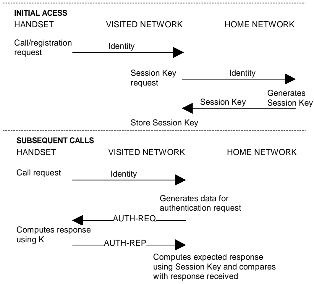
Figure D.2: Roaming using sessions keys
