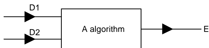
Figure 5.1: A algorithm
