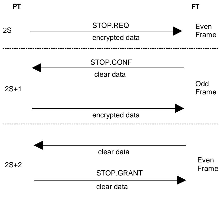
Figure 6.8: Encryption stop - good link example
