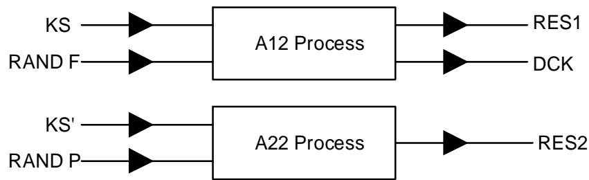
Figure 4.7: Derivation of RES1, DCK and RES2
