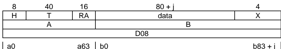
Figure 6.10: Half slot field structures
