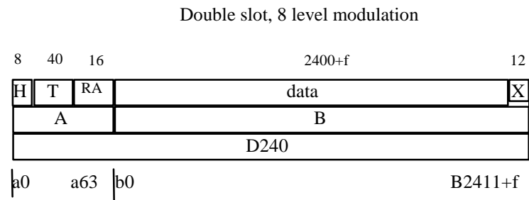
Figure 6.15: Unprotected B-field slot field structures for 4- and 8- level modulation slot formats
