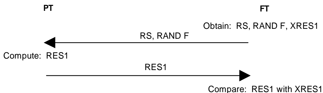
Figure 4.1: Authentication of PT
