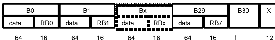
Figure 6.16: B-field multisubfield protected format for 4- and 8 level modulation formats
