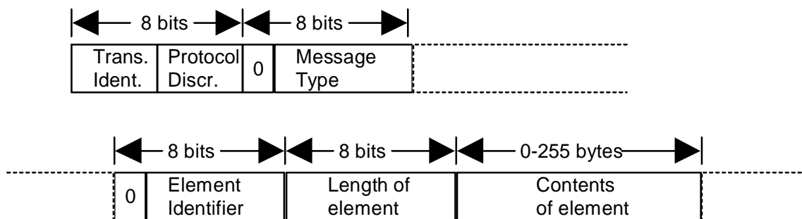
Figure 6.1: NWK Layer Message Structure (NLMS)
