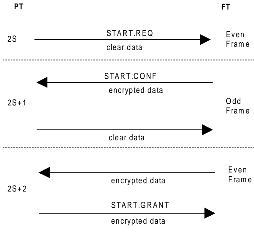
Figure 16: Encryption start - good link example
