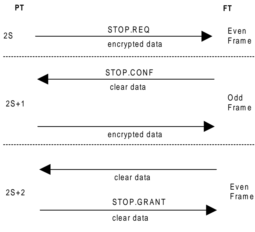
Figure 18: Encryption stop - good link example
