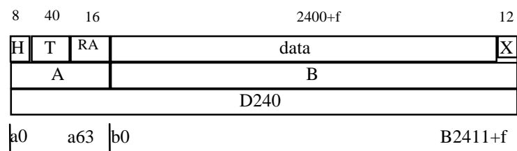
Figure 24: Unprotected B-field slot field structures for 4- and 8- level modulation slot formats
