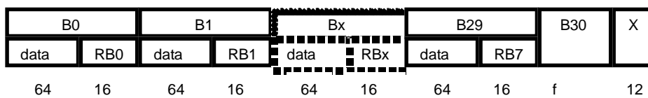
Figure 25: B-field protected format for 4- and 8 level modulation formats
