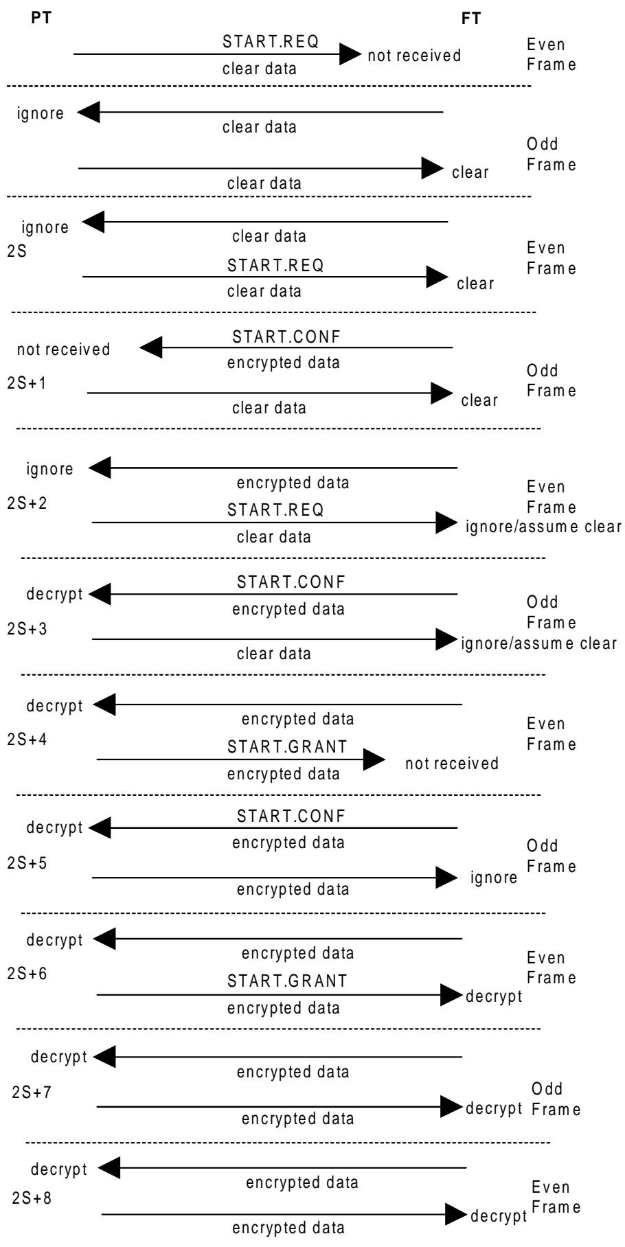
Figure 17: Encryption start - poor link example
