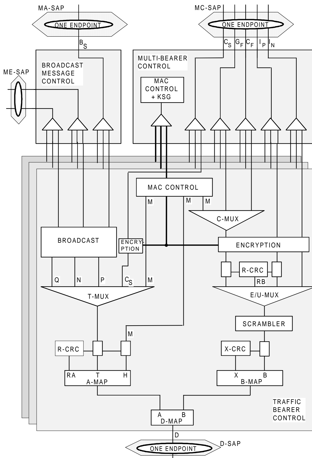
Figure 15: Placement of encryption
