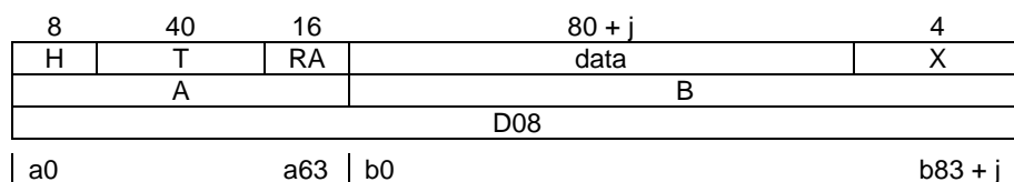
Figure 20: Half slot field structures
