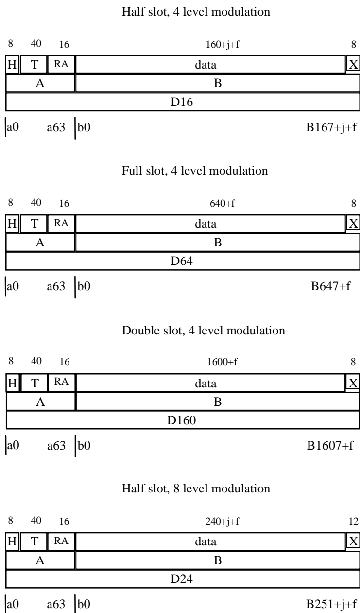
Figure 24 (continued): Unprotected B-field slot field structures for 4- and 8- level modulation slot formats
