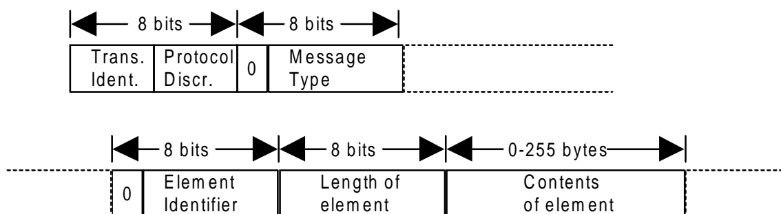
Figure 11: NLMS (NWK Layer Message Structure)
