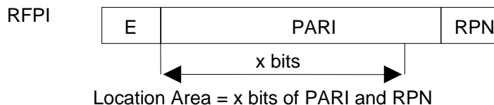
Figure 5.5: Location area with LAL = x bits
