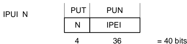
Figure 6.8: IPUI N
