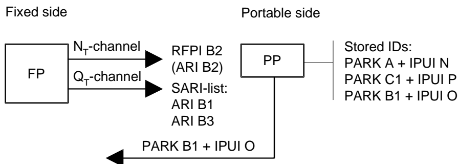
Figure A.6: Private ID usage (secondary)
