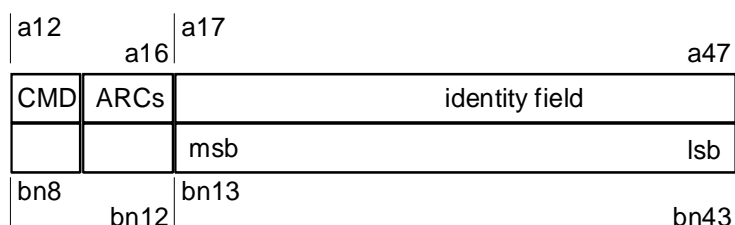
Figure 5.17: TARI FP response message
