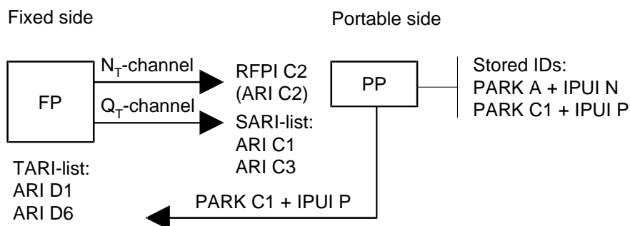
Figure A.3: Public ID usage (secondary)
