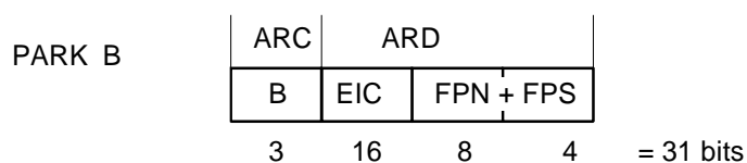
Figure 6.4: PARK B
