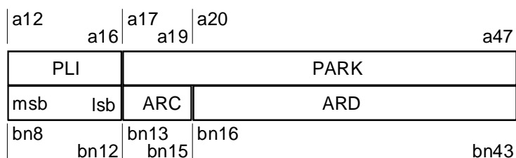
Figure 5.16: TARI PP request message
