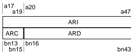
Figure 5.18: Identity field
