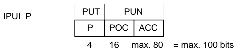
Figure 6.12: IPUI P
