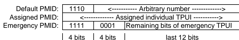
Figure 9.2: PMID structure
