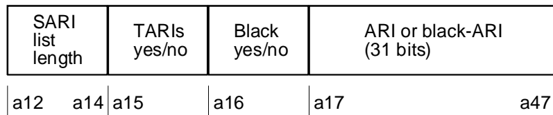
Figure 5.12: SARI message
