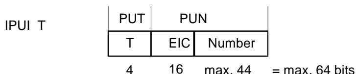
Figure 6.11: IPUI T
