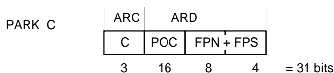
Figure 6.5: PARK C
