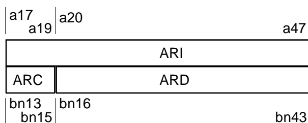
Figure 5.18: Identity field
