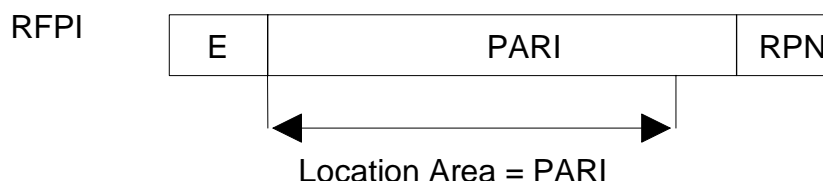
Figure 5.6: Default location area
