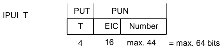
Figure 6.11: IPUI T
