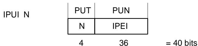
Figure 6.8: IPUI N
