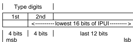
Figure 6.16: TPUI identity
