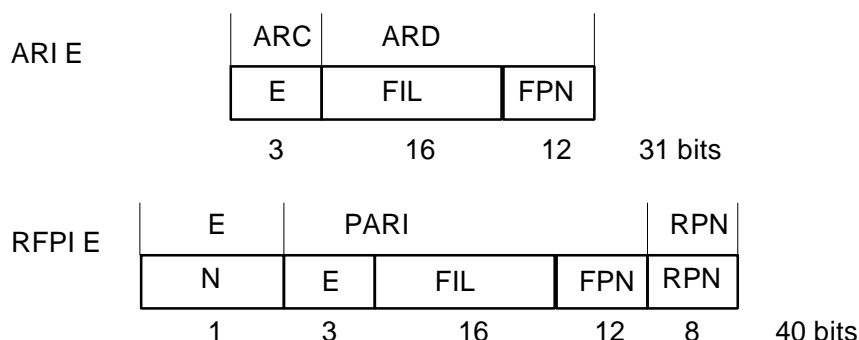
Figure 5.11: Access right class E, ARI, RFPI
