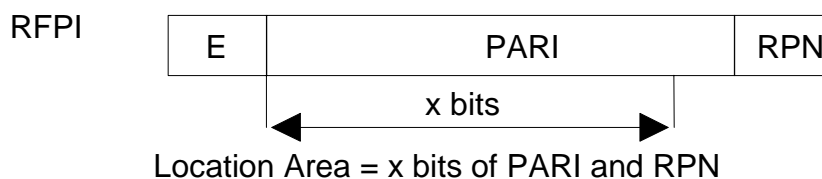
Figure 5.5: Location area with LAL = x bits
