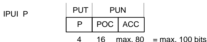
Figure 6.12: IPUI P
