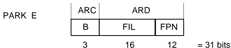
Figure 6.7: PARK E
