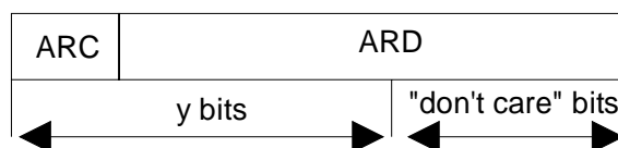
Figure 4.2: Structure of PARK\{y\}
