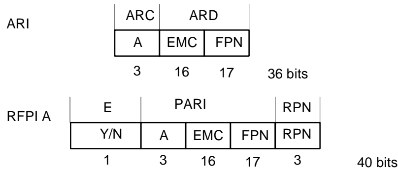
Figure 5.7: Access rights class A, ARI and RFPI
