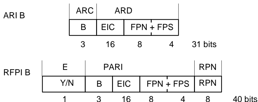
Figure 5.8: Access right class B, ARI, RFPI
