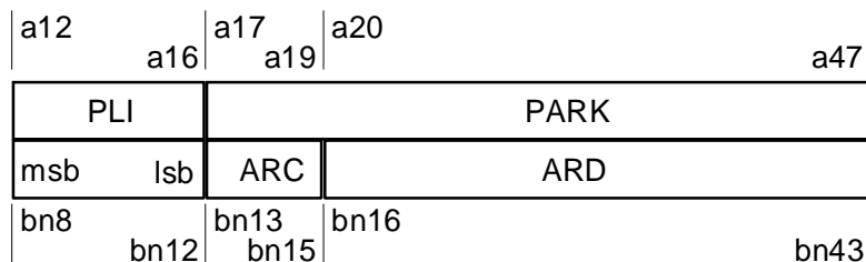
Figure 5.16: TARI PP request message
