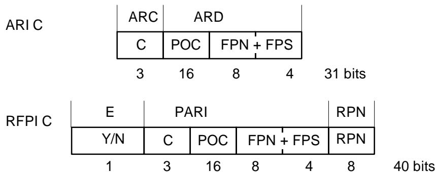
Figure 5.9: Access right class C, ARI, RFPI
