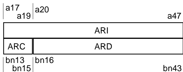
Figure 5.18: Identity field
