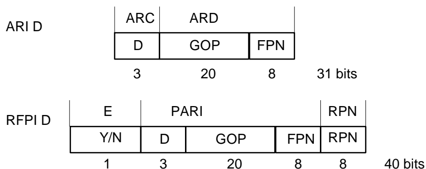
Figure 5.10: Access right class D, ARI, RFPI
