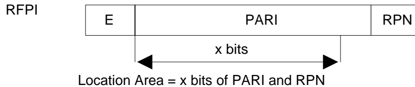
Figure 5.5: Location area with LAL = x bits
