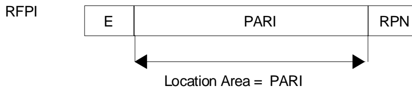
Figure 5.6: Default location area
