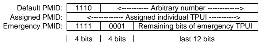
Figure 9.2: PMID structure
