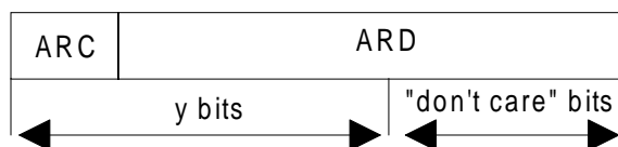
Figure 2: Structure of PARK\{y\}
