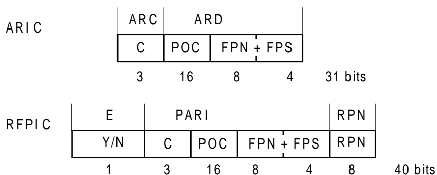
Figure 9: Access right class C, ARI, RFPI
