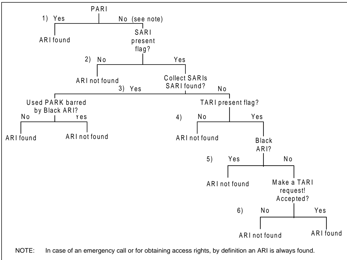
Figure 28: Procedure for a PP to find a suitable ARI
