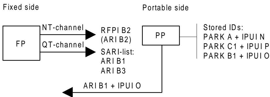
Figure A.6: Private ID usage (secondary)
