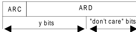
Figure 13: Structure of PARK{y}
