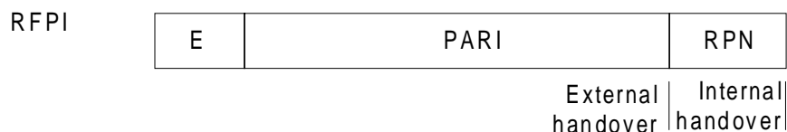
Figure 5: Indication of internal handover domain
