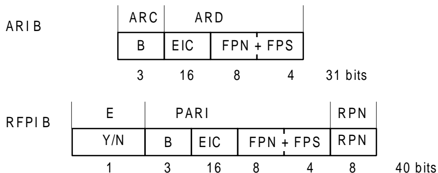
Figure 8: Access right class B, ARI, RFPI
