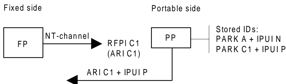
Figure A.2: Public ID usage (primary)
