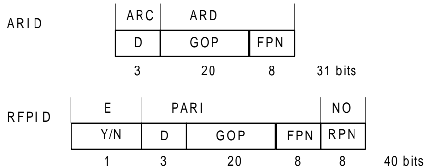
Figure 10: Access right class D, ARI, RFPI
