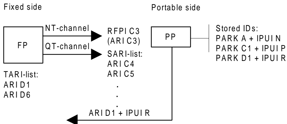
Figure A.4: Public ID usage (tertiary)
