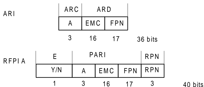
Figure 7: Access rights class A, ARI and RFPI
