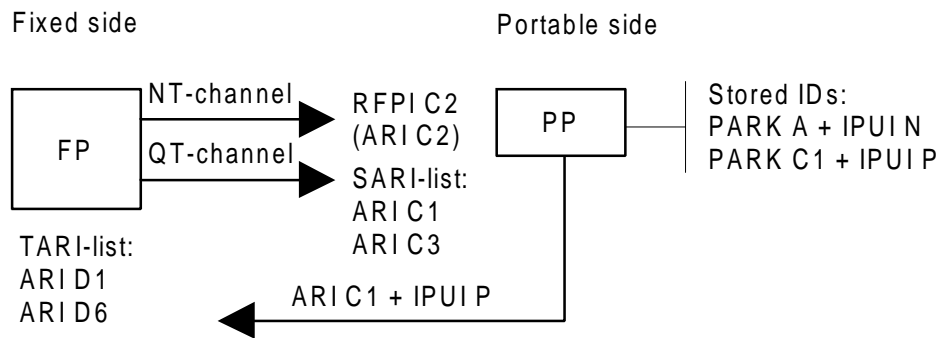
Figure A.3: Public ID usage (secondary)
