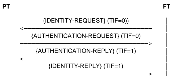
Figure H.1: Nested procedure, example 1
