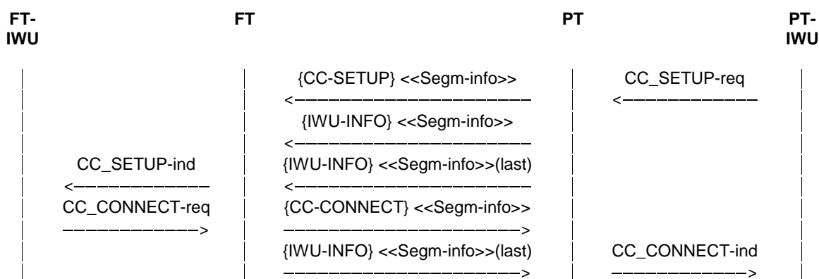
Figure 110c: Call setup with segmentation
