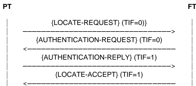
Figure H.2: Nested procedure, example 2
