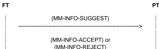
Figure 123a: FT parameter retrieval procedure (two way)
