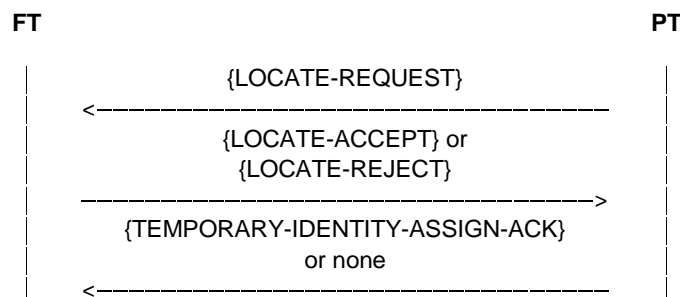
Figure 115: Location registration
