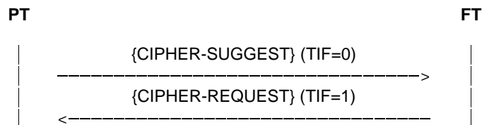
Figure H.6: PT initiated cipher switching, case 1
