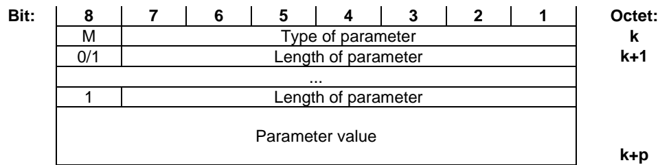
Figure 61c: Parameters fields' general structure
