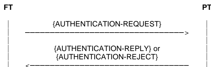
Figure 113: Authentication of the PT
