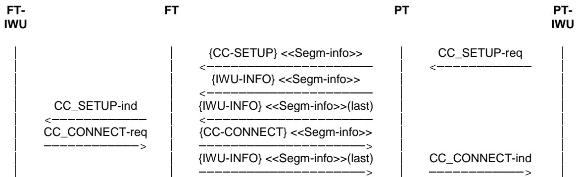
Figure 110a: Call setup with segmentation
