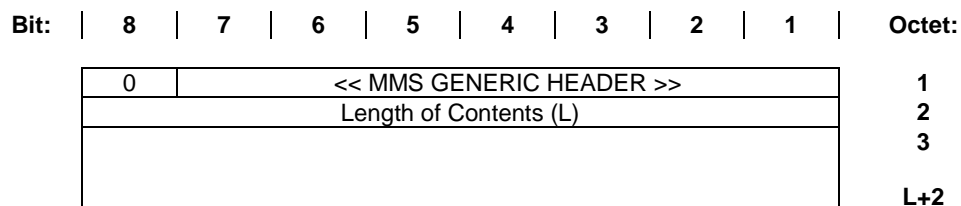
Figure 94: MMS GENERIC HEADER information element
