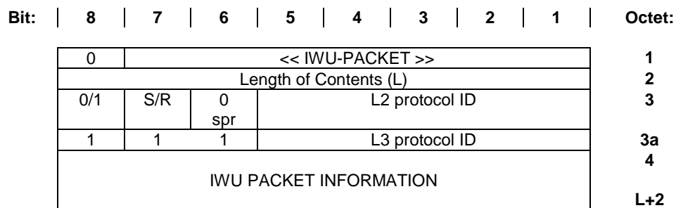
Figure 50: IWU-PACKET information element
