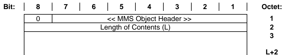
Figure 95: MMS OBJECT HEADER information element
