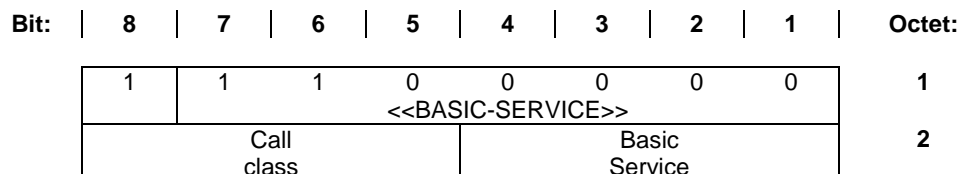
Figure 18: BASIC-SERVICE information element
