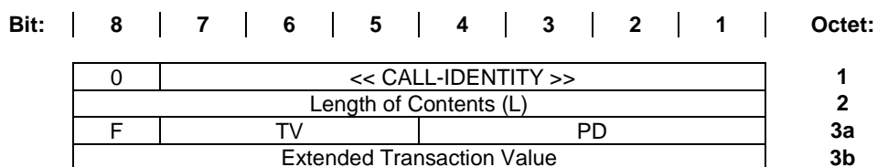
Figure 30: CALL-IDENTITY information element
