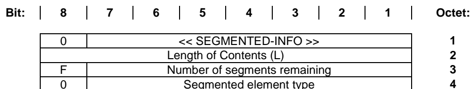
Figure 79: SEGMENTED-INFO information element
