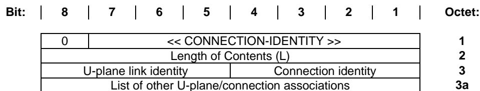
Figure 36: CONNECTION-IDENTITY information element
