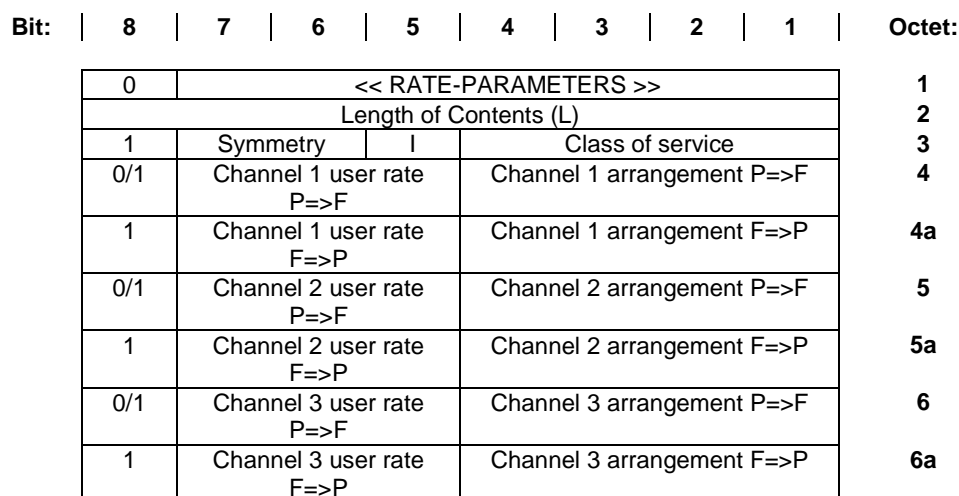
Figure 75: RATE-PARAMETERS information element
