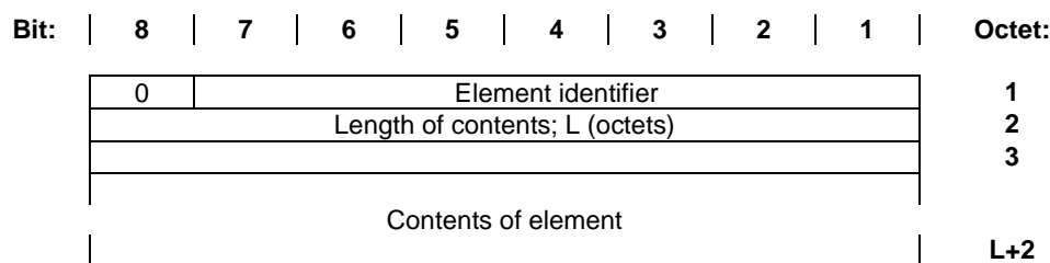
Figure 10: Variable length information element
