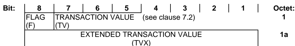
Figure 6: Extended Transaction Identifier (ETI) bits
