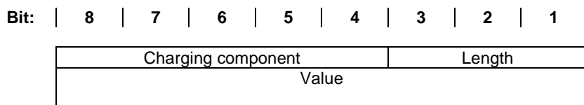
Figure 43: Cost information coding
