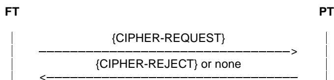
Figure 125: FT cipher switching
