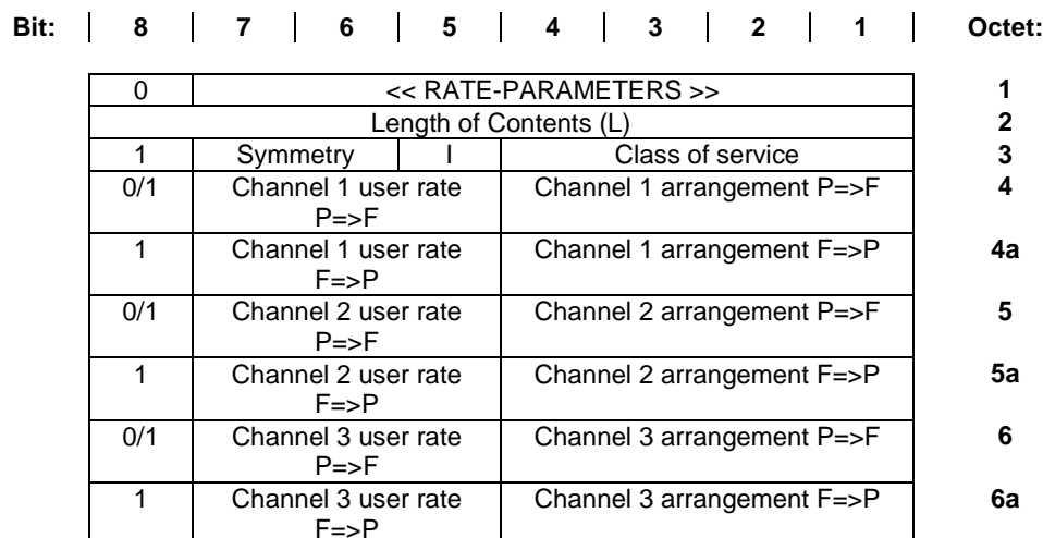
Figure 75: RATE-PARAMETERS information element
