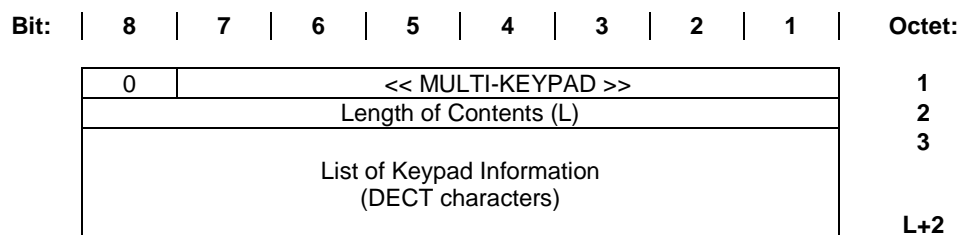
Figure 58: MULTI-KEYPAD information element
