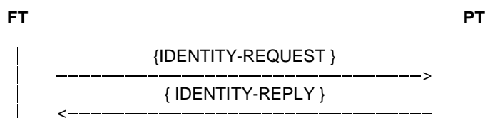
Figure 111: Procedure for identification of PT
