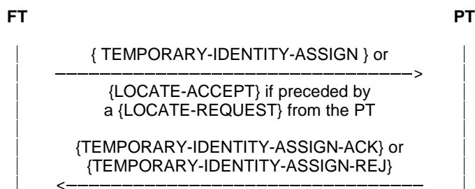
Figure 112: Temporary identity assignment
