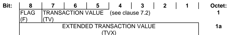
Figure 6: Extended Transaction Identifier (ETI) bits
