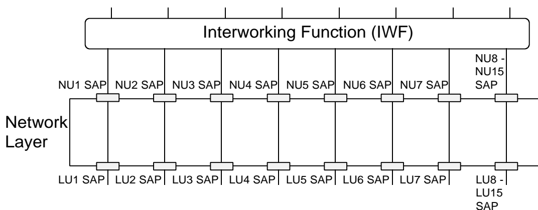
Figure 2: U-plane model
