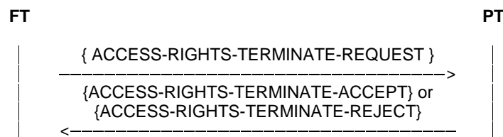
Figure 120: FT termination of access rights
