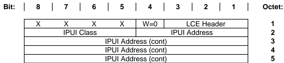
Figure 103: IPUI address structure
