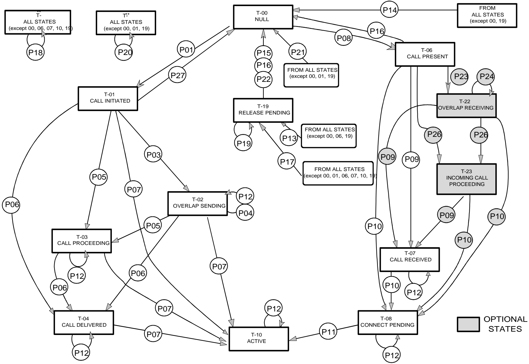
Figure 109: Call control states in the PT
