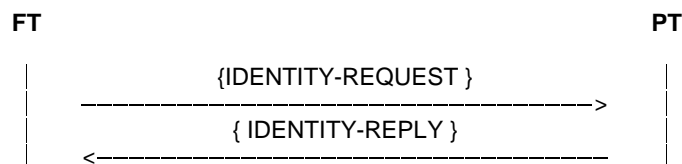
Figure 111: Procedure for identification of PT
