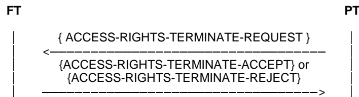
Figure 119: PT termination of access rights
